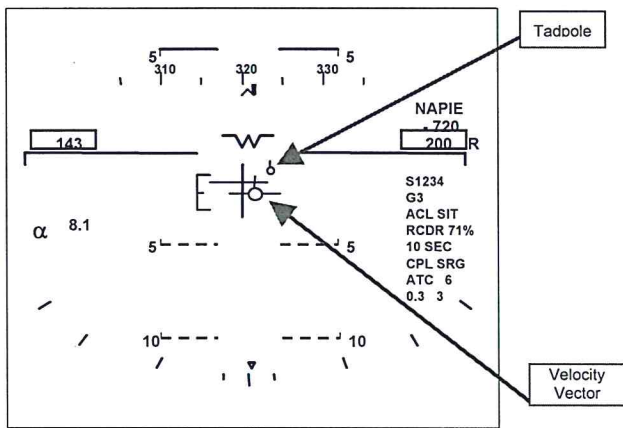
Figure 9 – SRGPS/NAPIE Head Up Display Illustration
