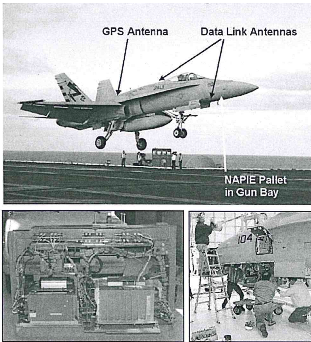
Figure 6 – F/A-18 Installation & SRGPS Pallet
