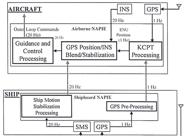
Figure 11 - SRGPS Functional Diagram
