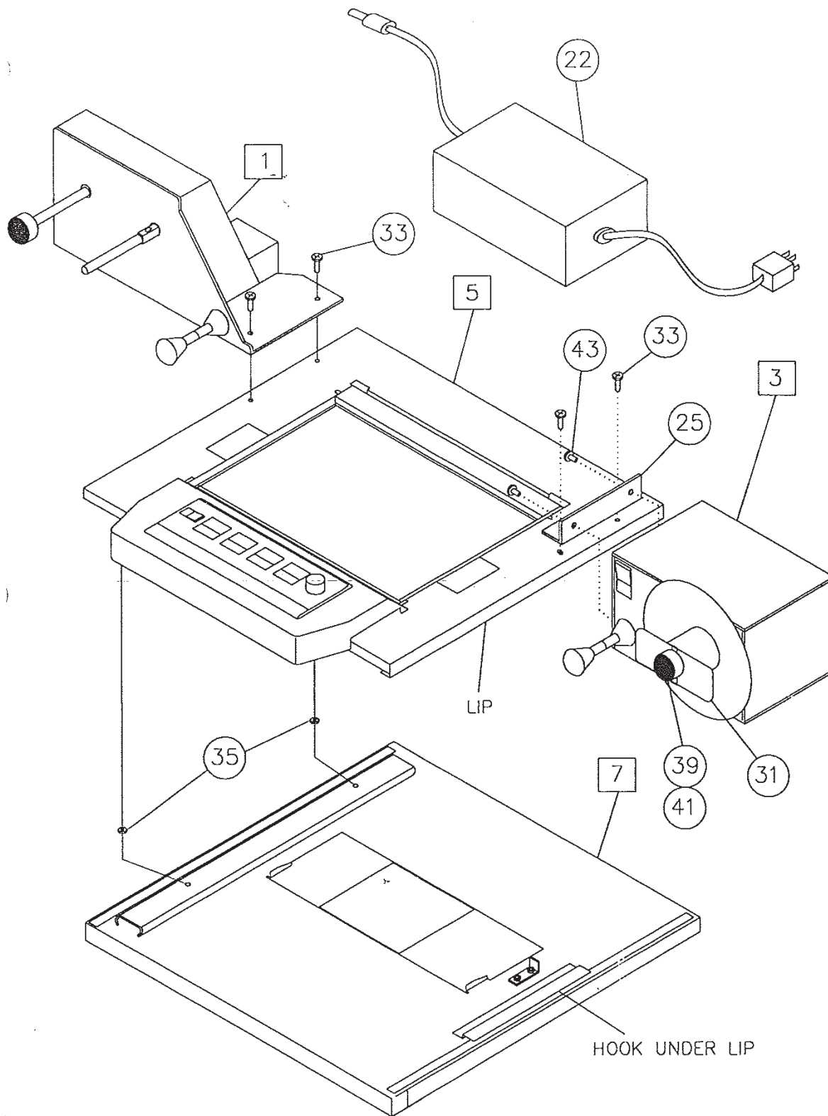
MOTORIZED COMBO SQUARED CARRIERS UC-6E 210000-01, UC-6EC 210000-02, UC-6ECM 210000-03
