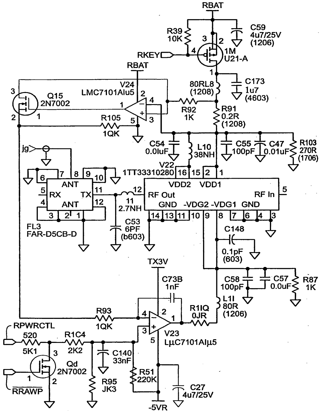
FIG. 5 Schematic for Current Control ALC
