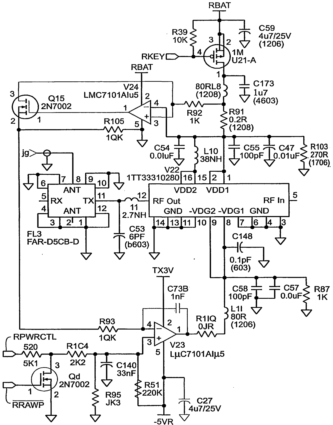
FIG. 5 Schematic for Current Control ALC
