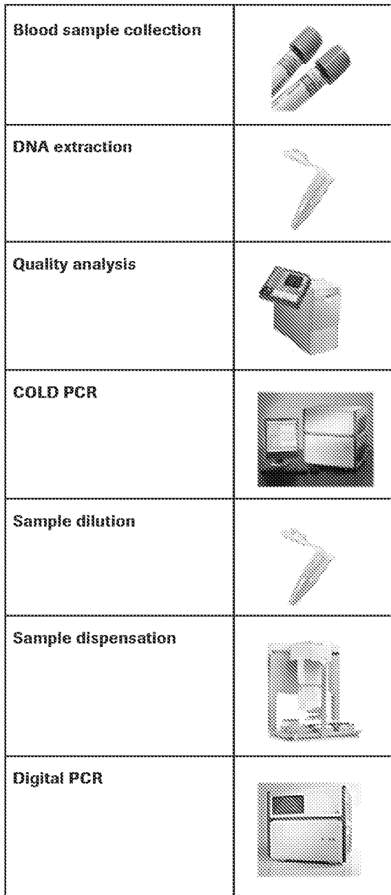
Figure 3: Workflow schematic for the detection of an IDH1 mutation in the plasma of glioma subjects
