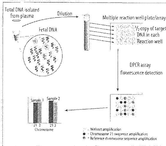
Figure 2. Digital PCR – For digital PCR (DPCR) the sample is diluted and distributed into a multi-reaction array (e.g. 384-well plate format) so that each reaction contains on average virtually \frac{1}{2} of a target molecule, or only every second reaction contains a target template. Subtle ratio differences, as in fetal aneuploidies, can be determined by counting positive PCRs of the target and reference sequence.
