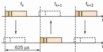
Figure 2 Frequency-hop/time-division-duplex channel.
