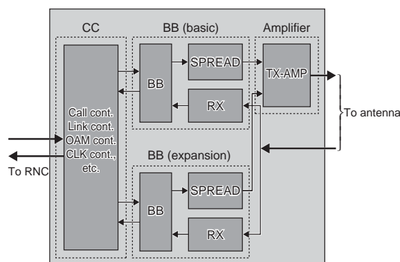
Figure 3 System configuration of large-capacity BTS.
