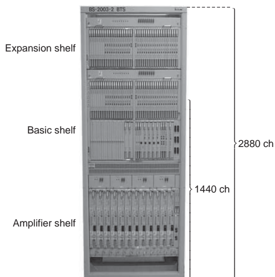
Figure 4 Shelf configuration of large-capacity BTS.
