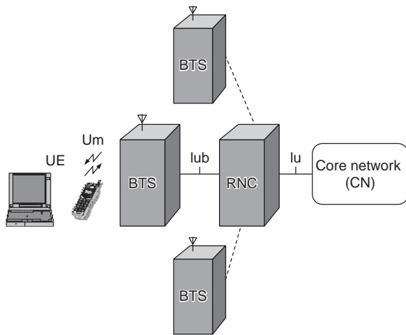
Figure 1 W-CDMA network configuration.
