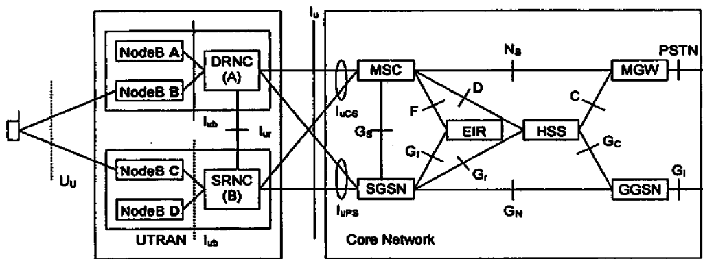
Figure 1: Network elements
