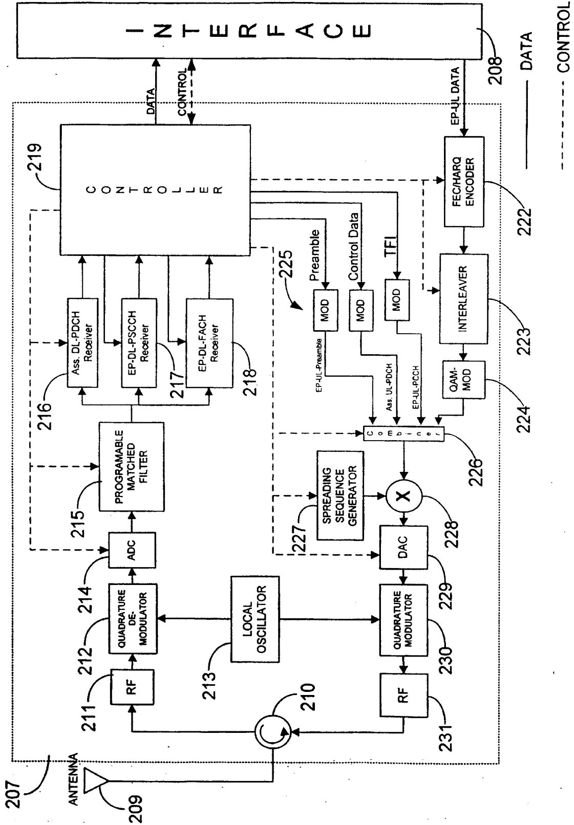
Fig. 15 Remote Station Transceiver for Enhanced Uplink Packet Communications.
