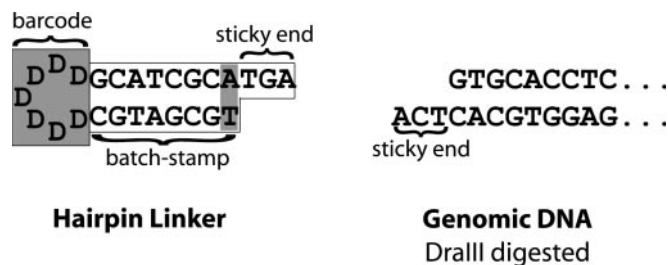
Figure 1. Schematic of barcoded and batch-stamped hairpin linker, designed for ligation to DraIII-cut genomic DNA of FMR1 . The letter D represents a nucleotide randomly selected from A, G and T.
