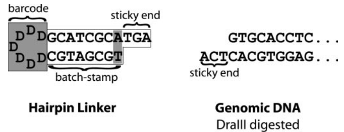
Figure 1. Schematic of barcoded and batch-stamped hairpin linker, designed for ligation to DraIII-cut genomic DNA of FMR1 . The letter D represents a nucleotide randomly selected from A, G and T.
