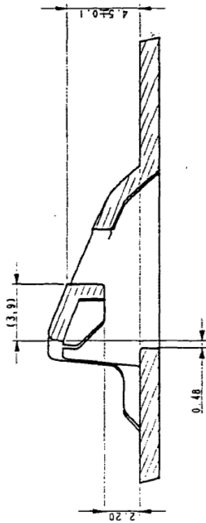
SECTION B-B SCALE 5:1
