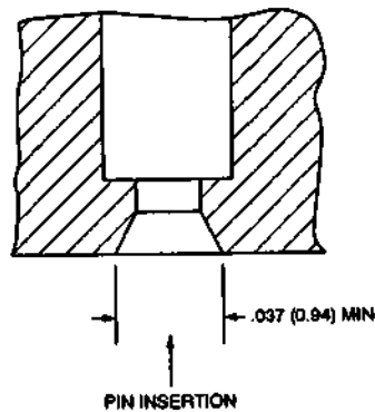
Figure 3-6. Card Connector Socket
