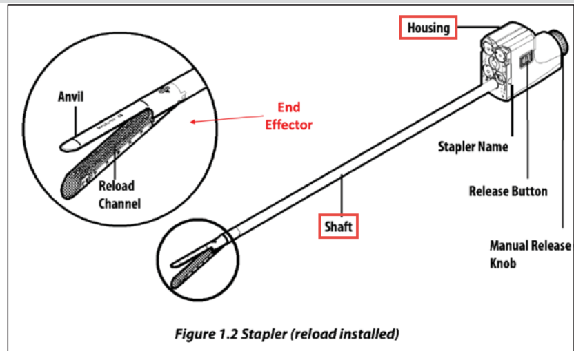
Figure 1.2 Stapler (reload installed) Exhibit 29 at p. 11 (annotations in red)
