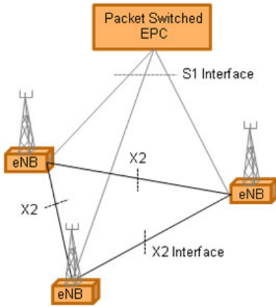
Figure 2. X2 and S1 Interfaces
