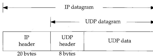
Figure 11.1 UDP encapsulation.
