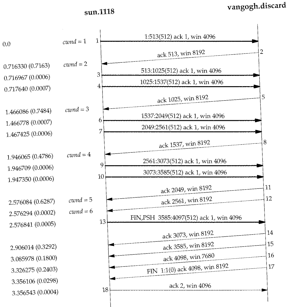
Figure 20.8 Example of slow start.
