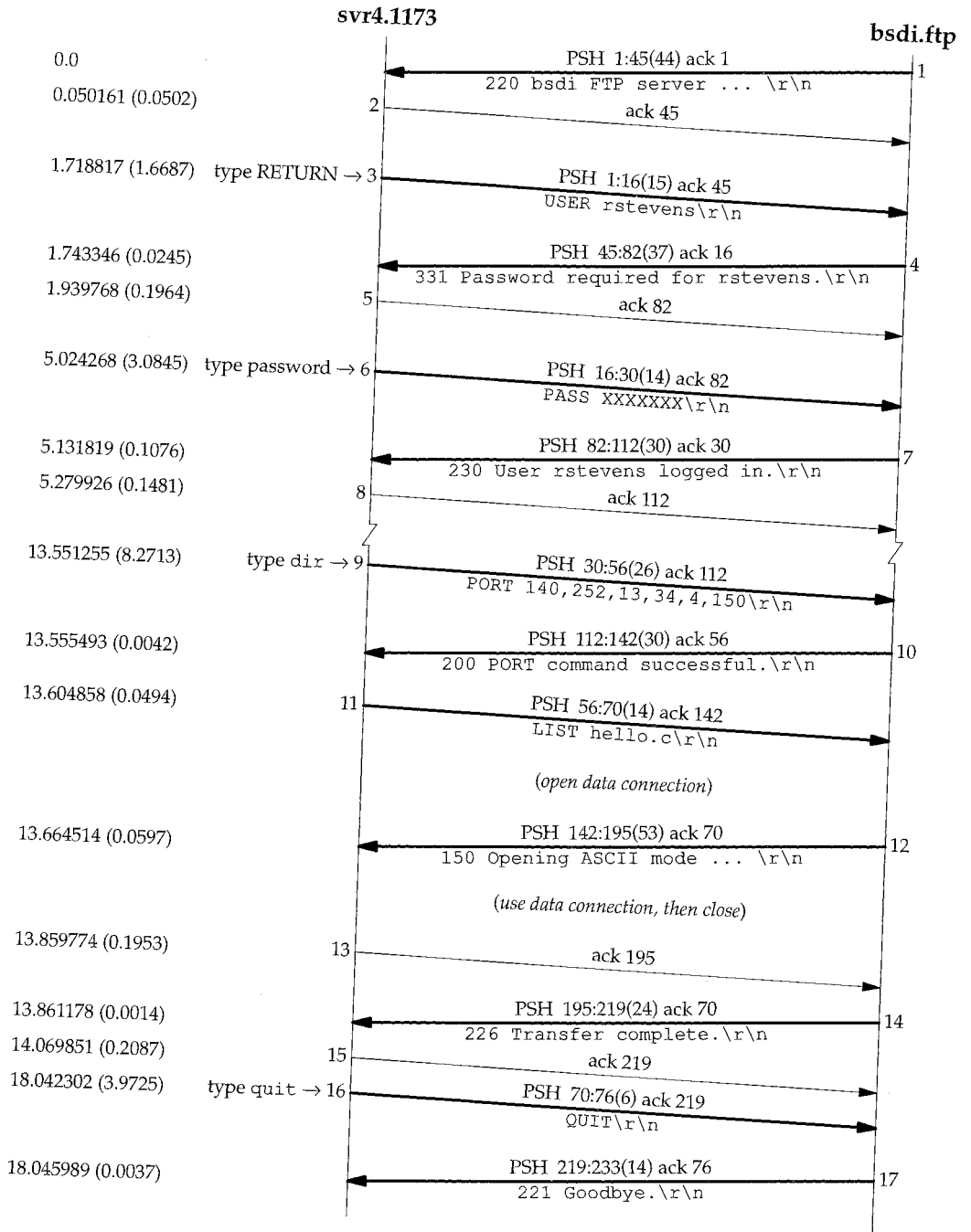
Figure 27.6 Control connection for FTP example.
