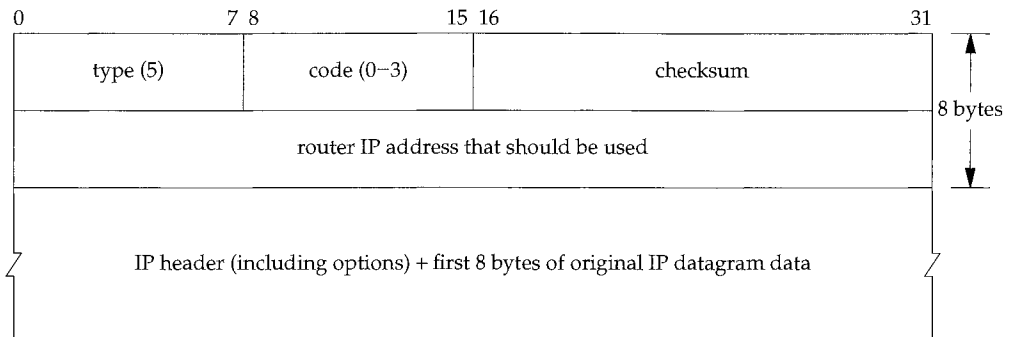
Figure 9.4 ICMP redirect message.
