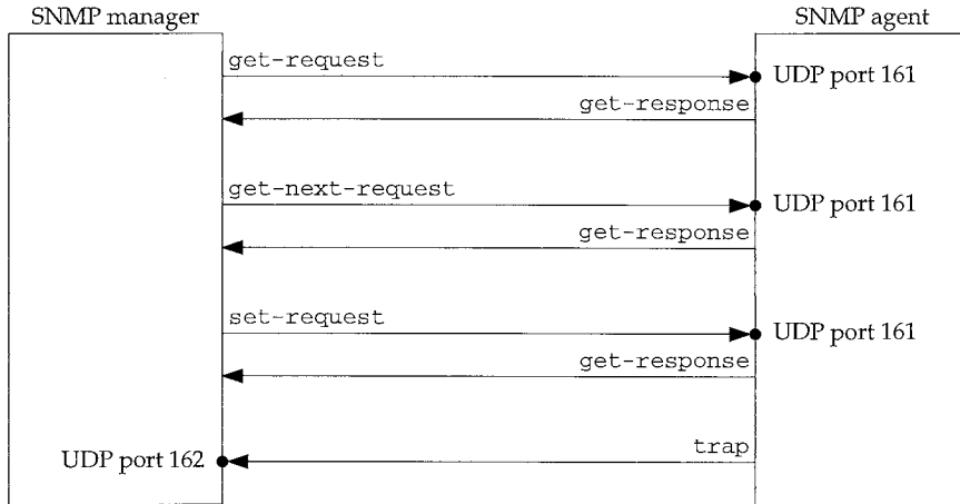
Figure 25.1 Summary of the five SNMP operators.
