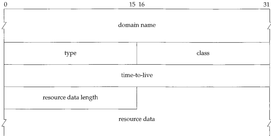
Figure 14.8 Format of DNS resource record.
