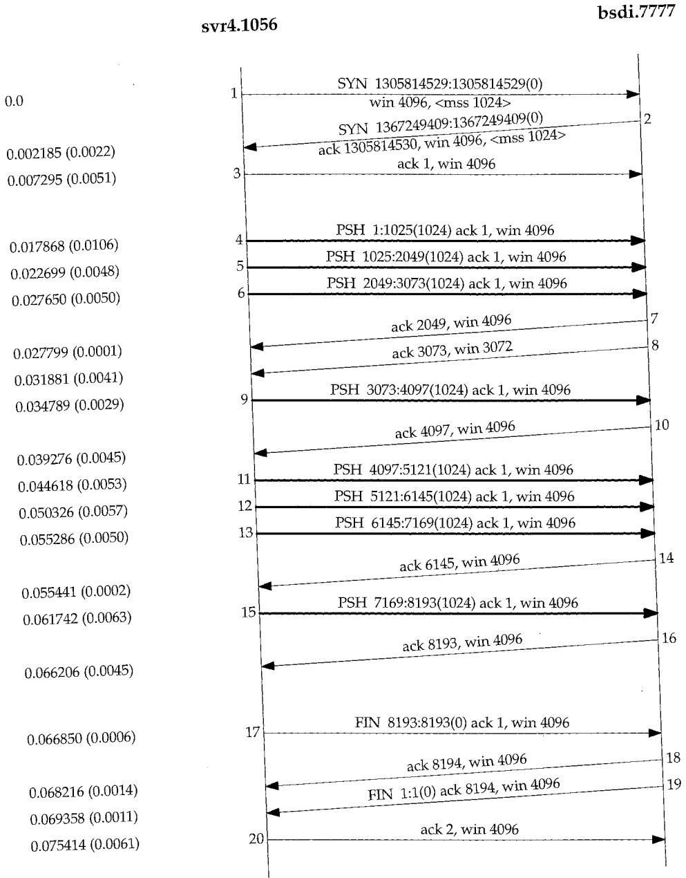
Figure 20.1 Transfer of 8192 bytes from svr4 to bsd1.
