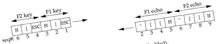
Figure 19.8 Time line for Figure 19.7 (Nagle algorithm disabled).
