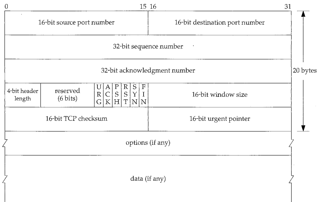
Figure 17.2 TCP header.
