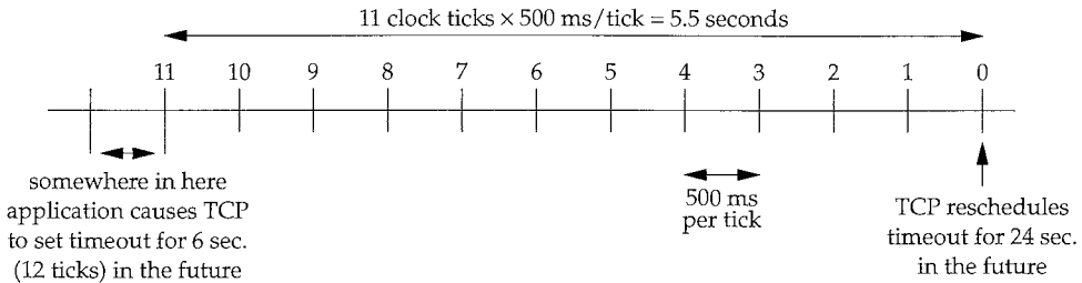
Figure 18.7 TCP 500-ms timer.
