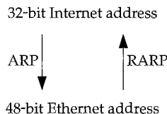
Figure 4.1 Address resolution protocols: ARP and RARP.
