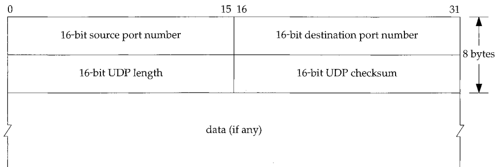
Figure 11.2 UDP header.
