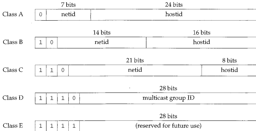
Figure 1.5 The five different classes of Internet addresses.
