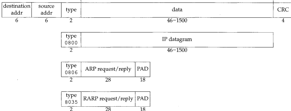
Figure 2.1 IEEE 802.2/802.3 encapsulation (RFC 1042) and Ethernet encapsulation (RFC 894).
