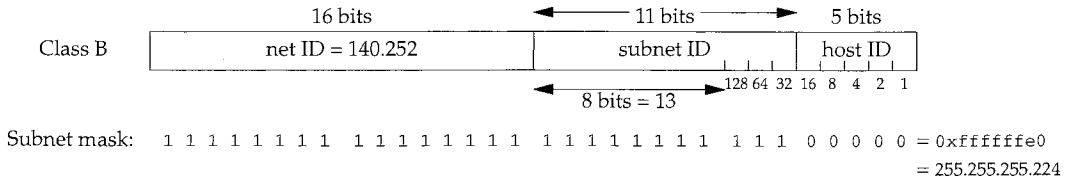
Figure 3.11 Using variable-length subnets.
