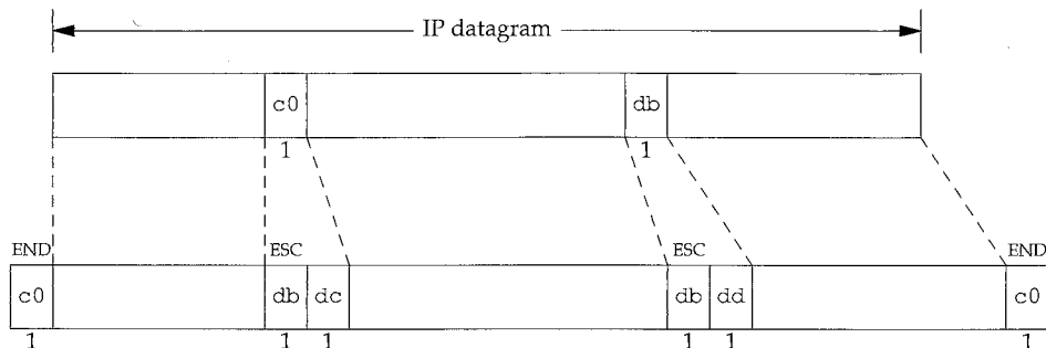
Figure 2.2 SLIP encapsulation.
