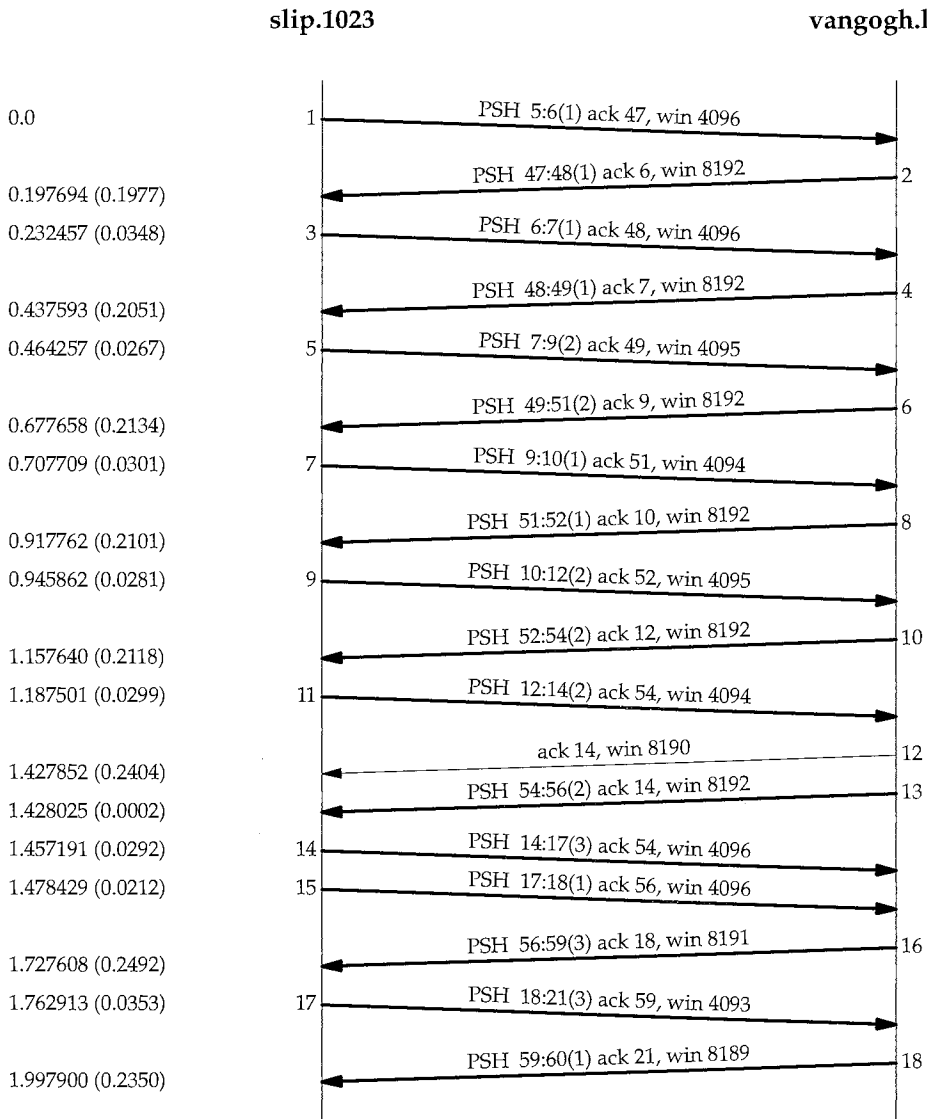
Figure 19.4 Data flow using rlogin between slip and vangogh.cs.berkeley.edu.
