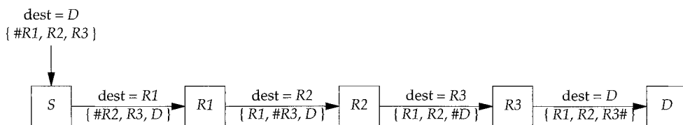
Figure 8.7 Example of IP source routing.
