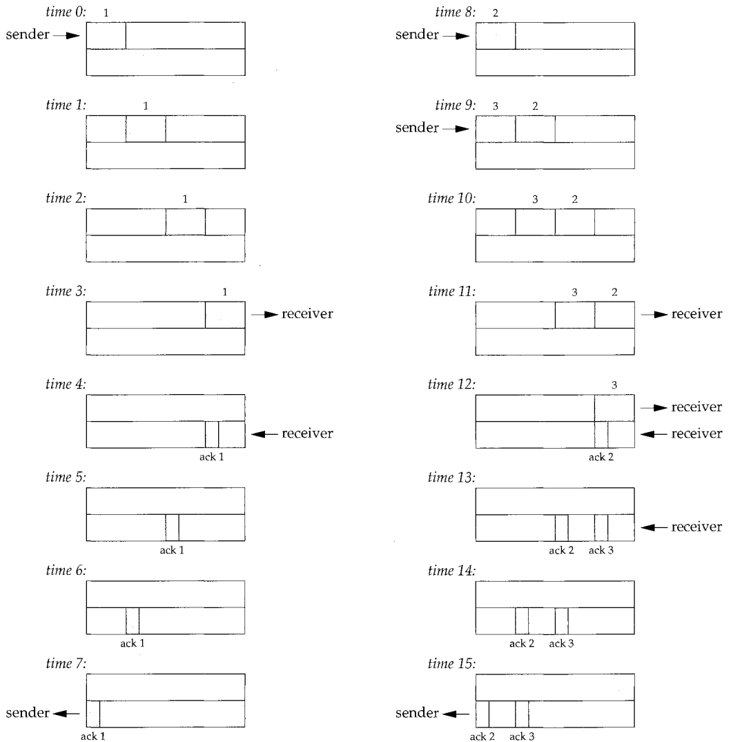
Figure 20.9 Times 0–15 for bulk data throughput example.
