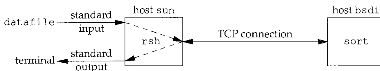
Figure 18.11 The command: rsh bsd1 sort < datafile .
