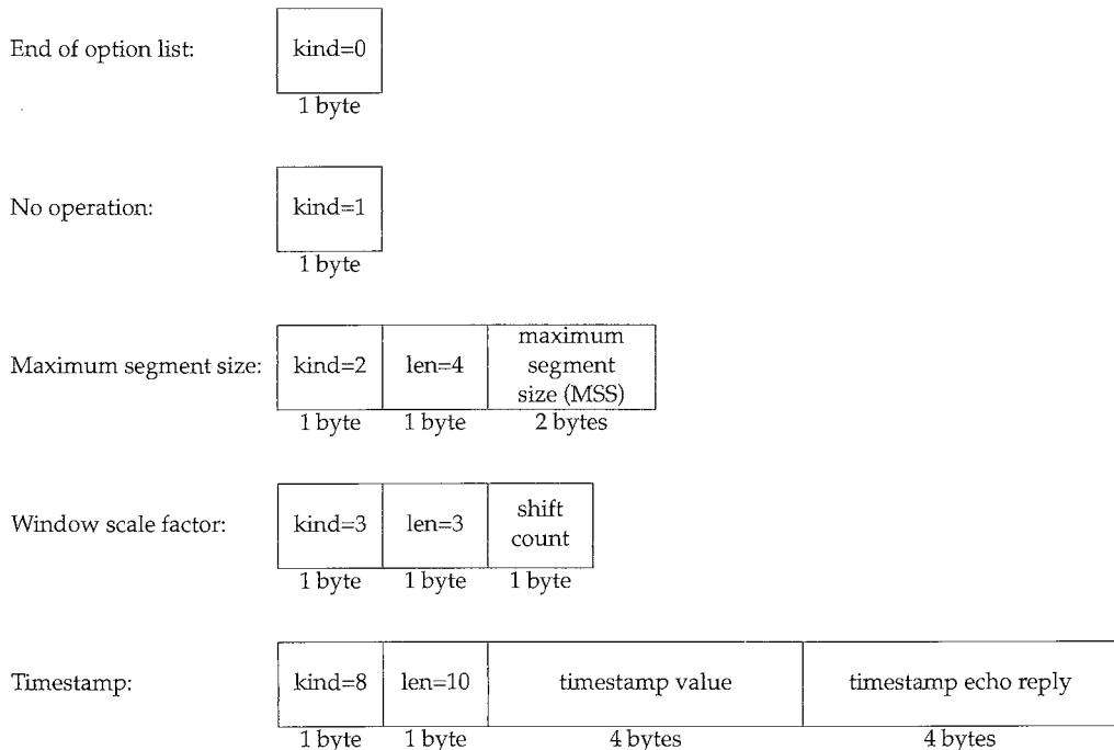
Figure 18.20 TCP options.
