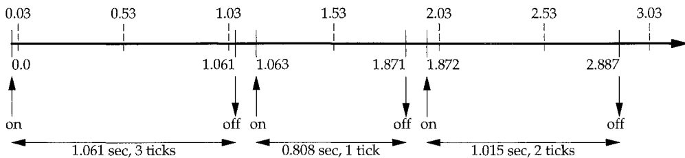
Figure 21.3 RTT measurements and clock ticks.
