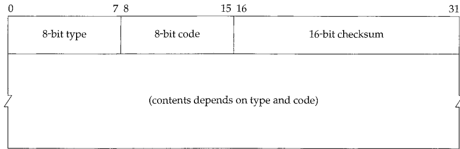
Figure 6.2 ICMP message.
