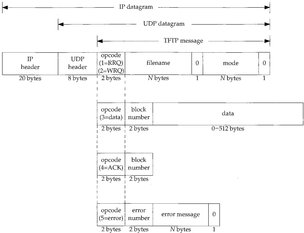
Figure 15.1 Format of the five TFTP messages.
