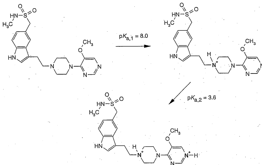
Fig. 9. Protonation of avitriptan corresponding to its two \text{p}K_a values
