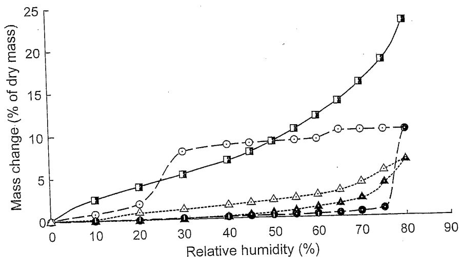
Fig. 15. Water vapor sorption isotherms of three salts of a basic investigational compound. \circ : Hydrochloride, \Delta : hydrogen tartrate, \square : hydrogen malonate (sorption and desorption without hysteresis); black symbols: adsorption; empty symbols: desorption.
