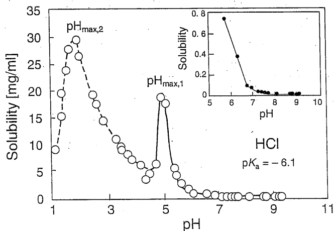
Fig. 10. \text{pH} -Solubility profile of avitriptan at 25^\circ\text{C} where HCl was used to adjust \text{pH} , indicating two \text{pH}_{\text{max}} values. Solubility profile at \text{pH} above 5 is shown in the inset.
