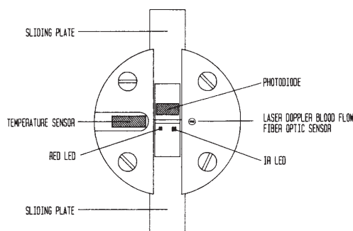
Fig. 2. Frontal view of the combined SaO 2 /laser Doppler skin blood flow sensor.
