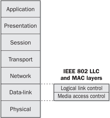
IEEE 802.x. ISO/OSI reference model with IEEE 802 LLC and MAC layers shown.
