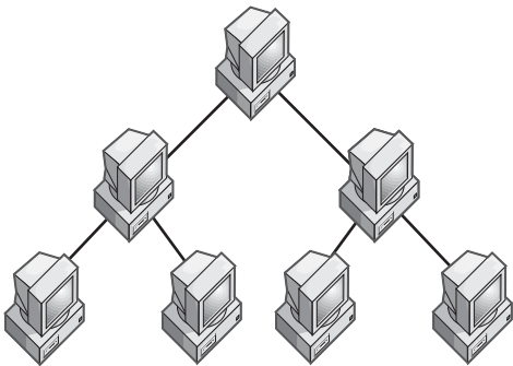
Tree network.
