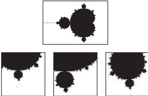
Fractal.
