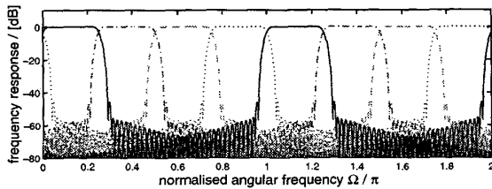
Fig. 5: Magnitude response of K = 8 channel filter bank decimated by N = 6 .
