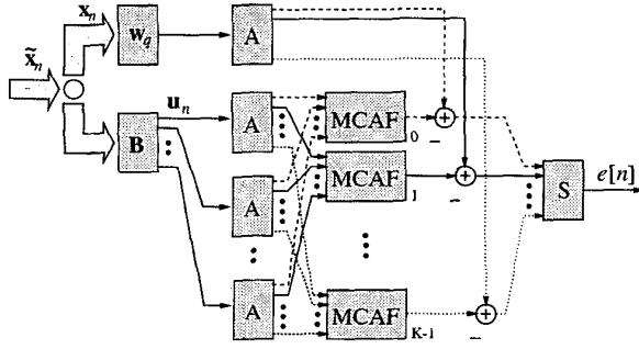
Fig. 4: Subband adaptive GSC; an independent MCAF is applied to each subband.
