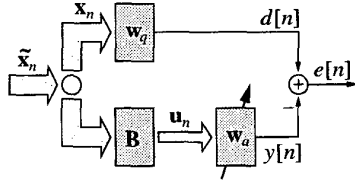
Fig. 2: Structure of a generalized sidelobe canceller.
