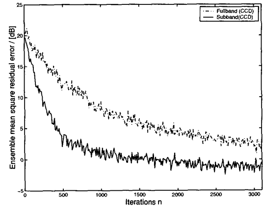
Fig. 7: Learning curves for simulation II ( S = 2 ).
