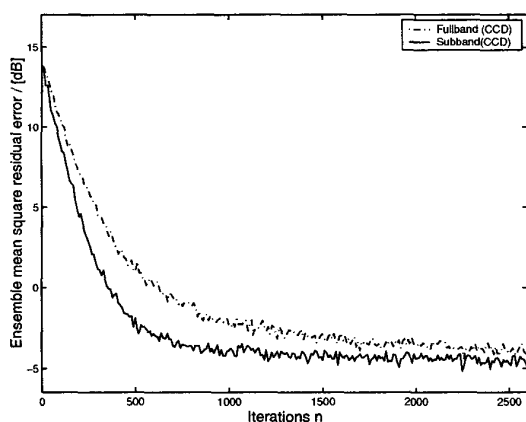
Fig. 9: Learning curves for simulation IV ( S = 1 ).
