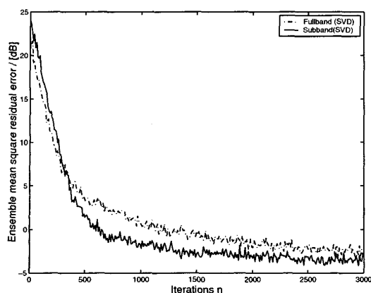
Fig. 8: Learning curves for simulation III ( S = 1 ).
