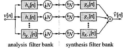
Fig. 3: K channel filter banks with decimation N .
