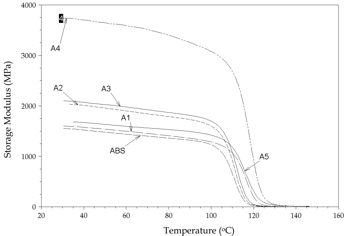
Figure 5-17: Storage Modulus of Various Copper/ABS Composites with copper particle size of 10 \mu\text{m} at Temperature Scan
