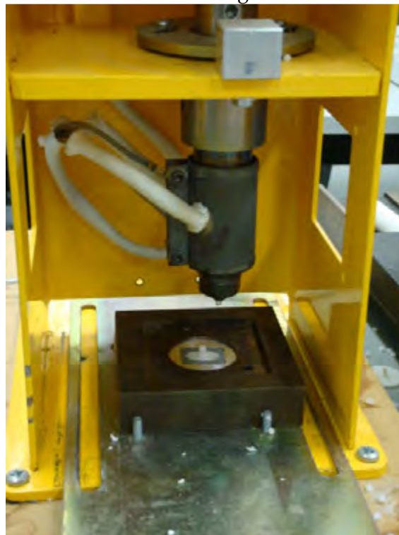
Figure 7-13: Mini tool insert fabricated on FDM fitted into steel blade for injection moulding
