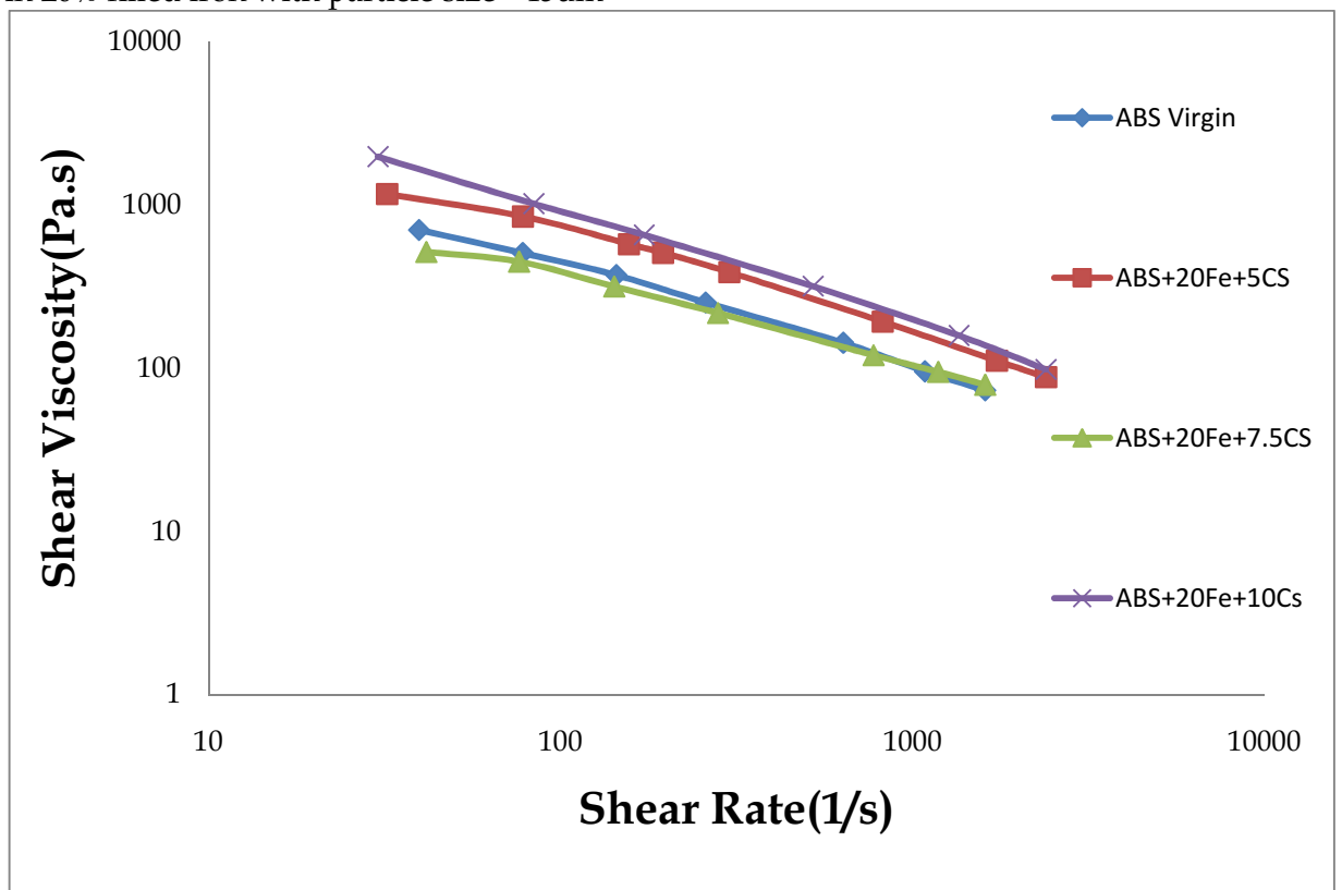
Figure 4-20: Flow curves of composites of ABS and varying volume fractions of Ca.St. in 20% filled iron with particle size <45um
