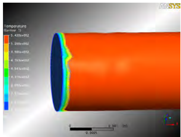
Figure 6-23: 3D Temperature evolution at the inlet using CFX
