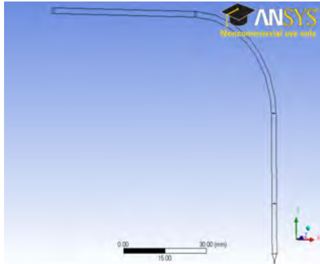
Figure 6-10: Internal features of liquefier used in FDM3000
