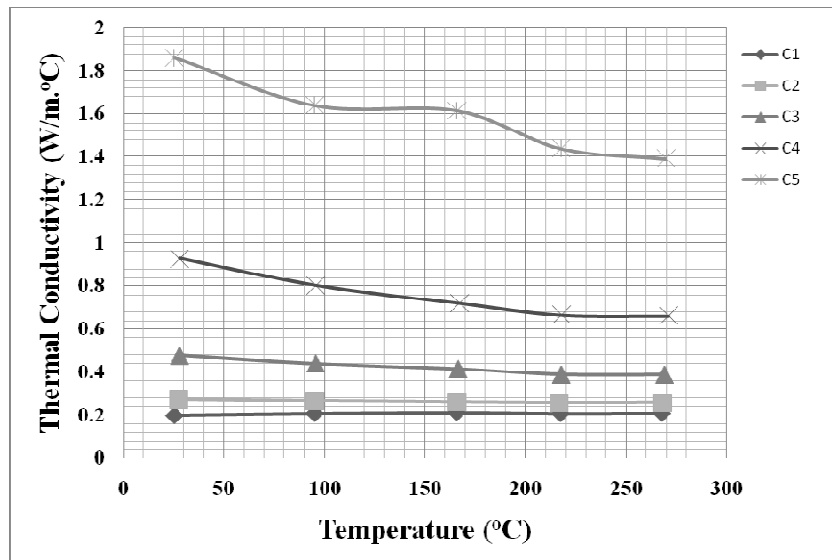
Figure 5-28: Thermal Conductivity of iron filled ABS composite for various temperatures
