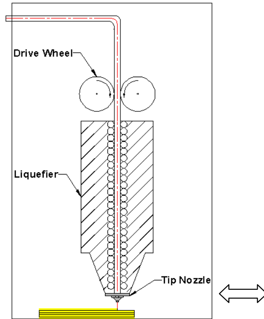
Figure 2-10: FDM Liquefier Straight Nozzle
