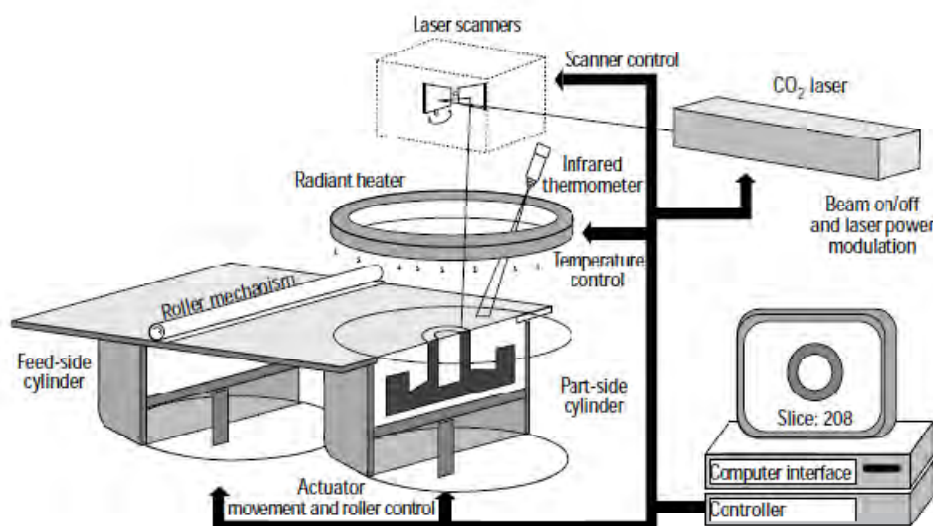
Figure 2-6: Illustration of the SLS process (Subramanian et al. 1995)
