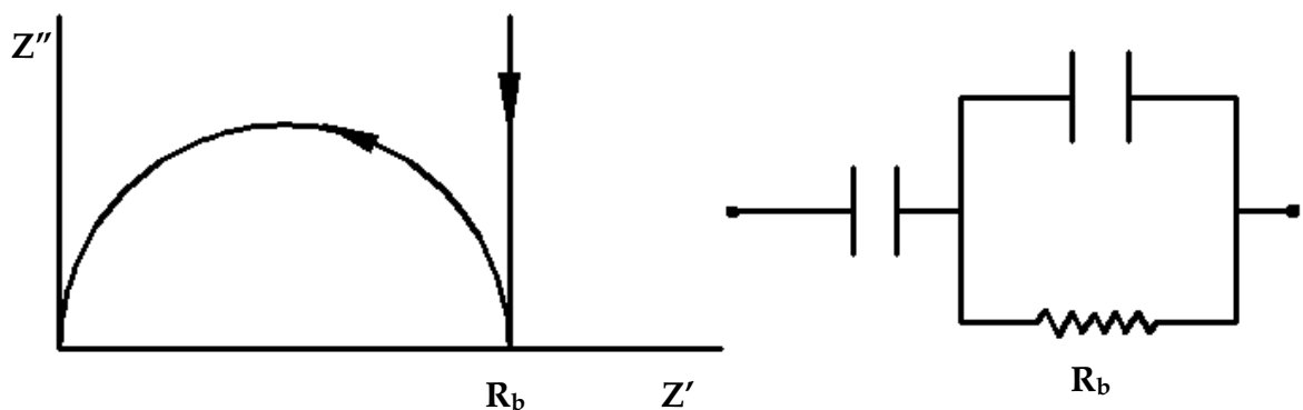
Figure 5-32: A typical simple Nyquist plot and its equivalent circuit
