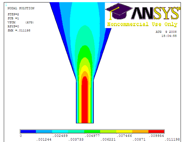
Figure 6-21: Maximum velocity at the nozzle exit
