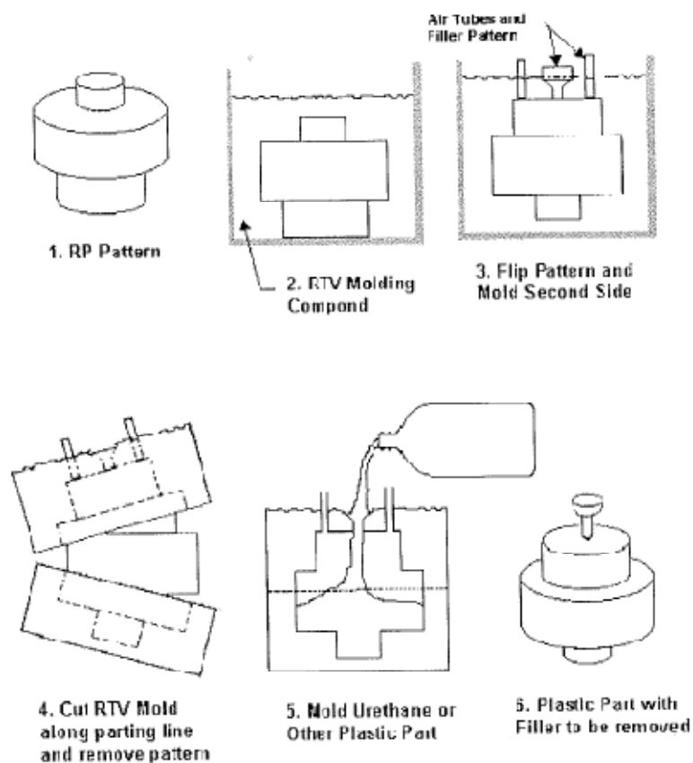
Figure 2-5: Illustration of Silicon RTV moulding process (Grenda 2006)
