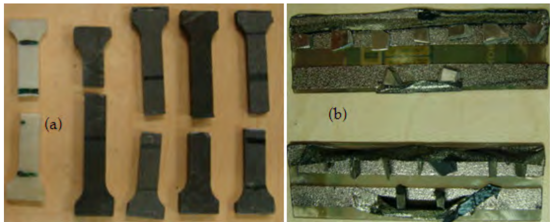
Figure 5-8: (a) Fractured tensile specimen (b) Samples prepared for SEM
