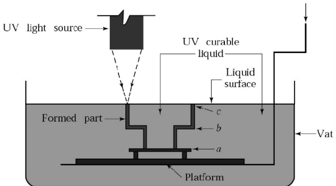
Figure 2-3: Schematic of Stereolithography process (Source: Ultra Violet Products, Inc)
