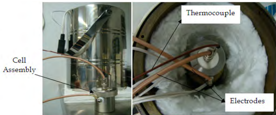
Figure 5-31: The cell setup used for Impedance spectroscopy in CSIRO
