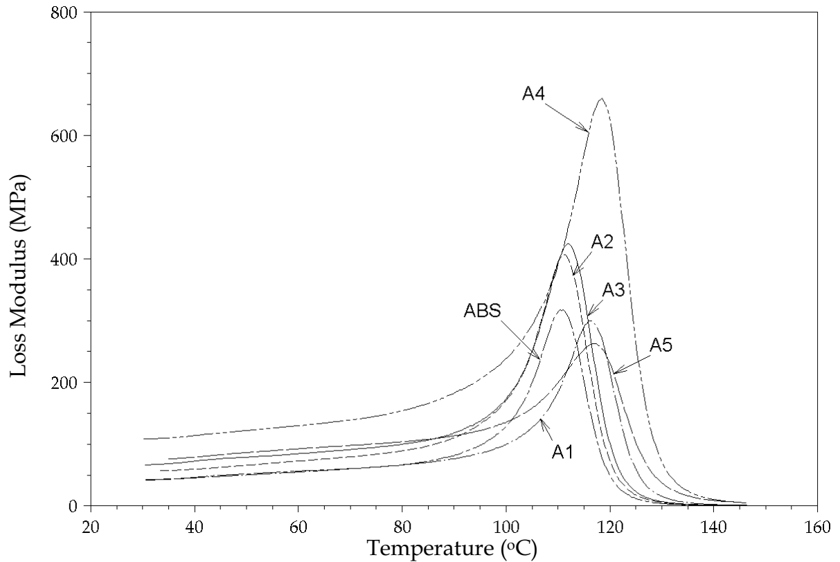
Figure 5-18: Loss Modulus of Various Copper/ABS Composites with copper particle size of 10 \mu\text{m} at Temperature Scan
