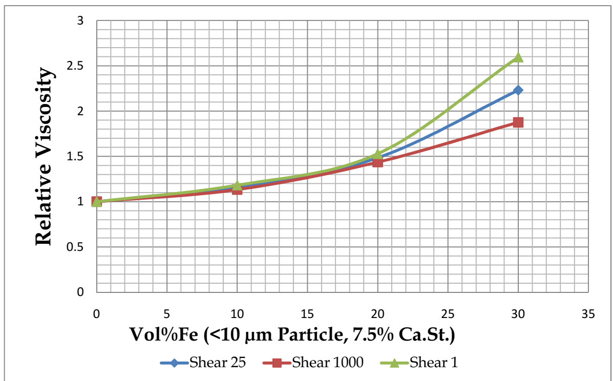
Figure 4-28: Relative viscosity of composites of ABS and varying volume fractions of Fe for 7.5 % Ca.St.
