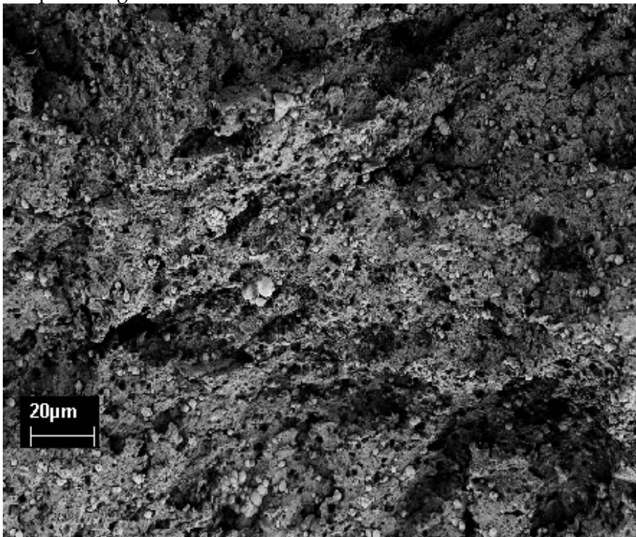
Figure 5-14: SEM image of fracture surface ABS-Fe(20 vol%) prepared by melt compounding
