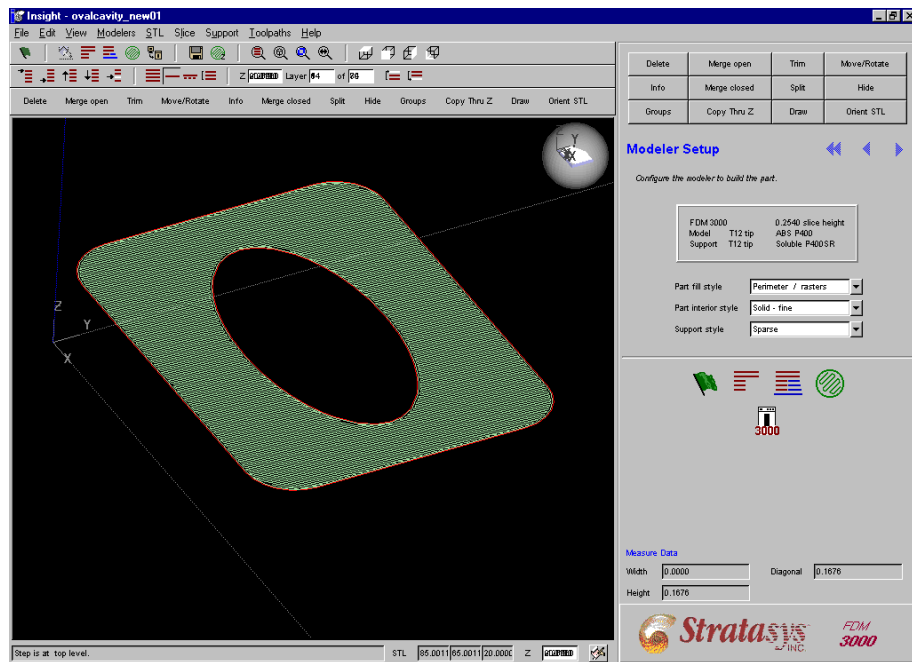
Figure 7-9: Generated tool path shown for the top layer of model
