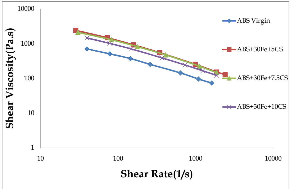
Figure 4-23: Viscosity vs. shear rate for various composites of ABS and Ca.St in 30% filled iron with particle size <45um
