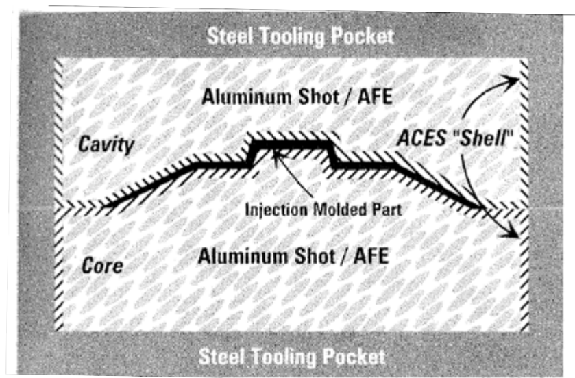
Figure 2-4: Illustration of Direct AIM "Shelling" backfilled with Al-filled Epoxy (Jacobs 2000)
