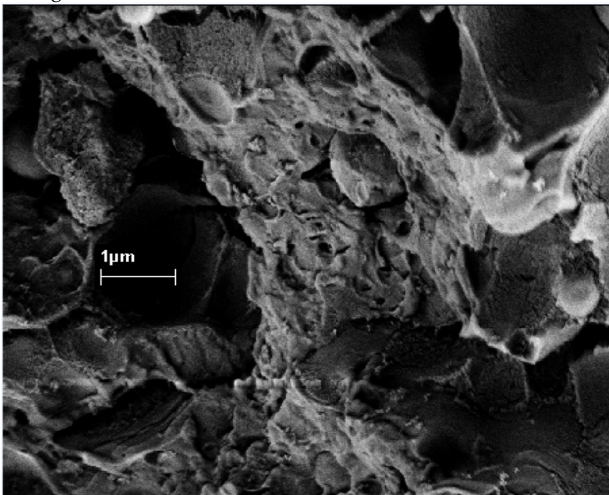
Figure 5-12: SEM image of fracture surface ABS-Fe(30 vol%) prepared via centrifugal mixing
