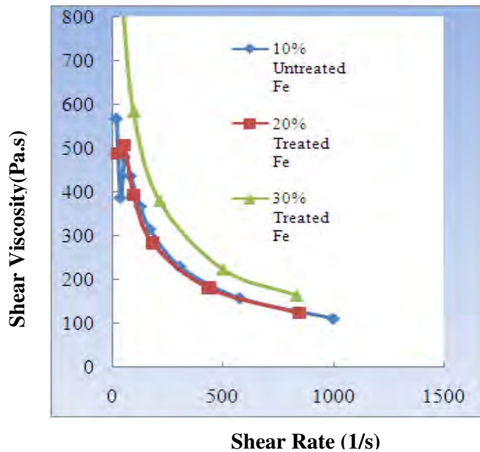
Figure 6-5: Apparent viscosity vs apparent shear rate
