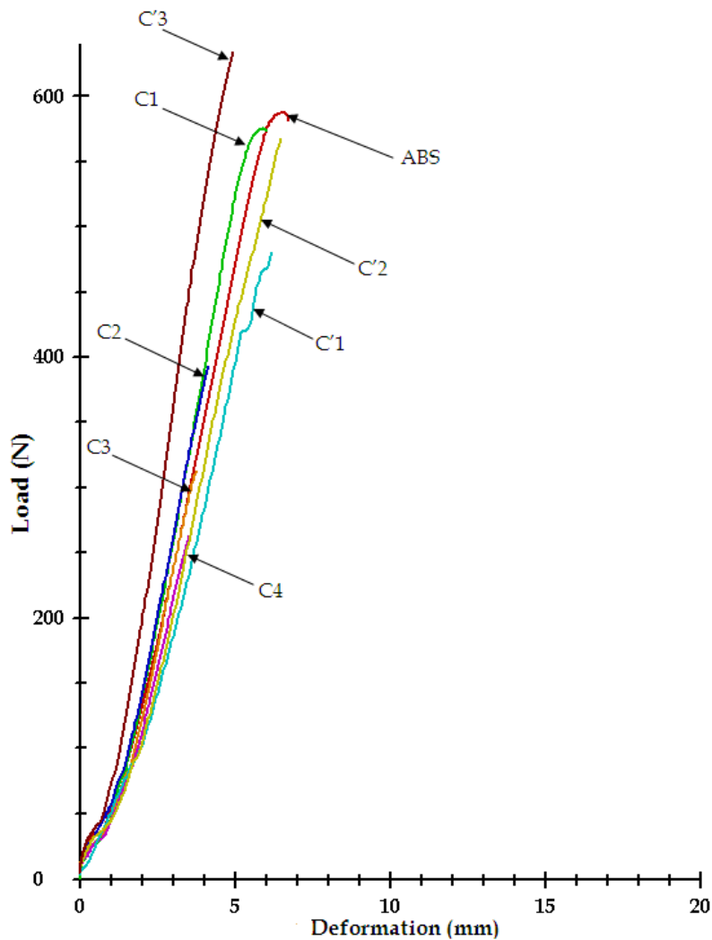
Figure 5-7: Load vs deformation behaviour of ABS-Iron Composites prepared by melt compounding on a twin screw extruder for various volume fraction of Iron powder
