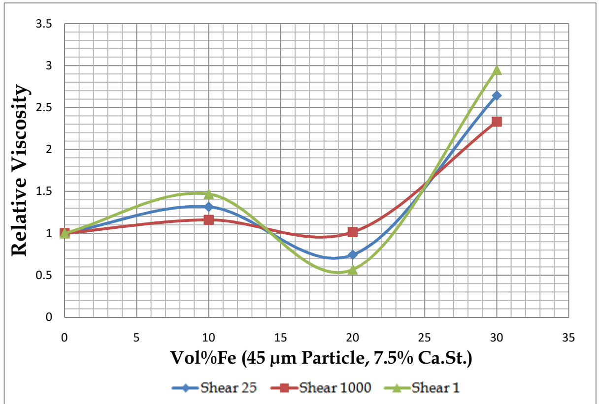
Figure 4-25: Relative viscosity of composites of ABS and varying volume fractions of Fe of 45 μm and 7.5% Ca.St.
