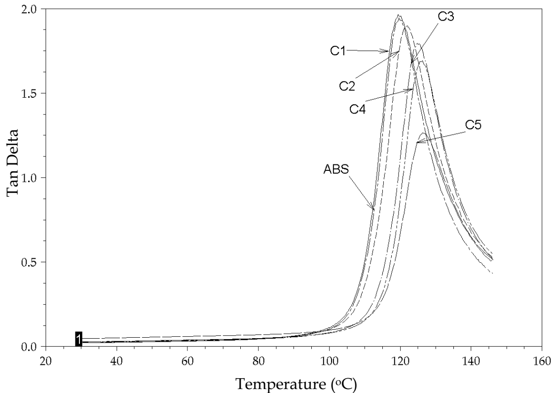
Figure 5-24: Tan Delta of Various Iron/ABS Composites with iron particle size of 45 \mu\text{m} at Temperature Scan
