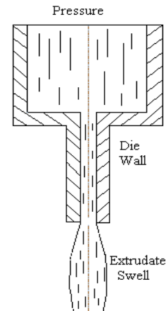
Figure 4-6: Schematic of Polymer Melt Swell
