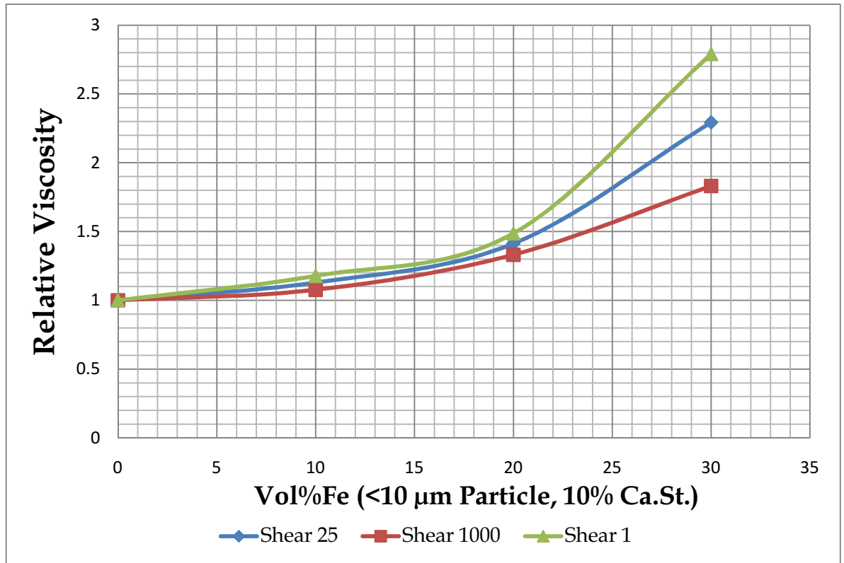
Figure 4-29: Relative viscosity of composites of ABS and varying volume fractions of Fe for 10% Ca.St.
