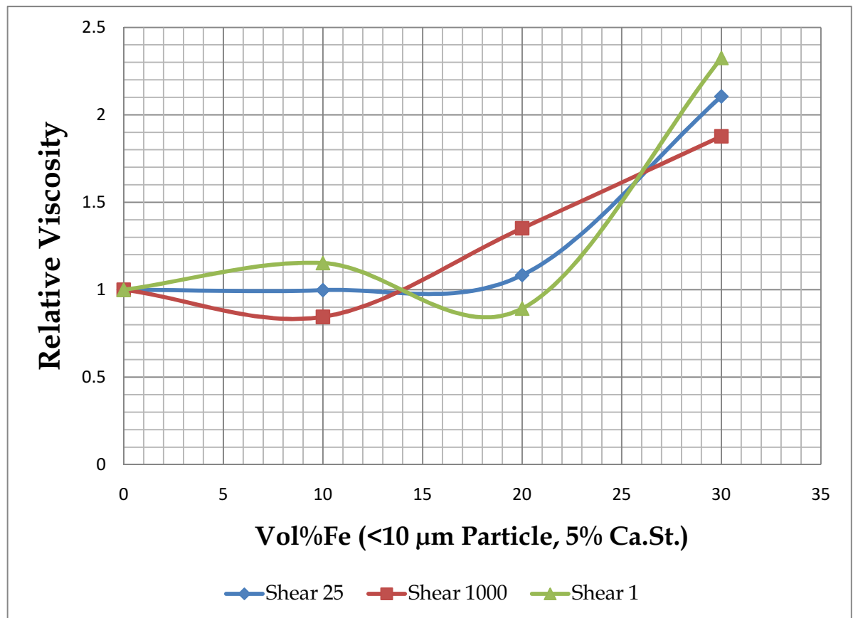
Figure 4-27: Relative viscosity of composites of ABS and varying volume fractions of Fe for 5% Ca.St.
