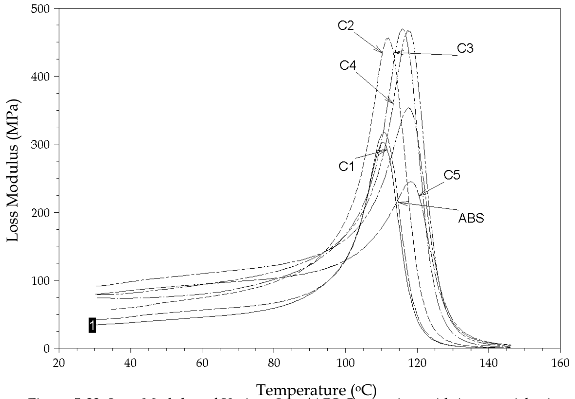
Figure 5-23: Loss Modulus of Various Iron/ABS Composites with iron particle size of 45 \mu\text{m} at Temperature Scan
