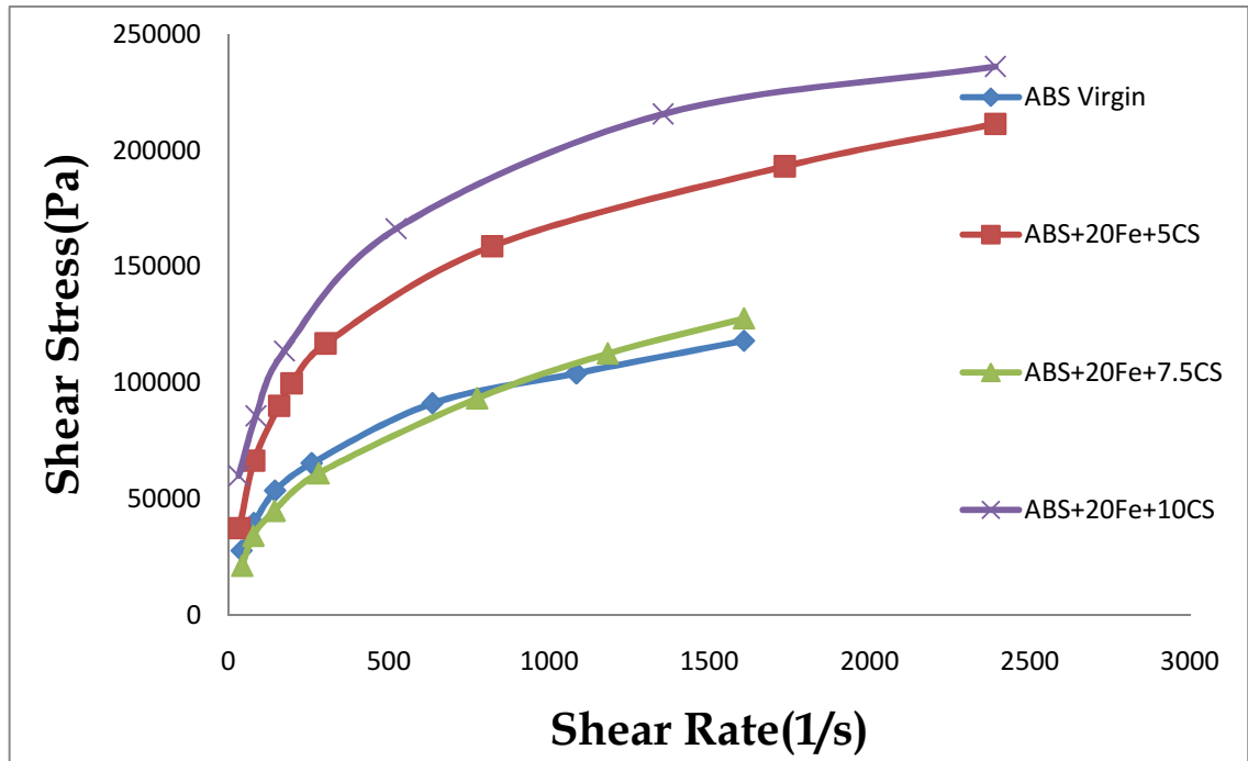
Figure 4-20: Flow curves of composites of ABS and varying volume fractions of Ca.St. in 20% filled iron with particle size <45um
