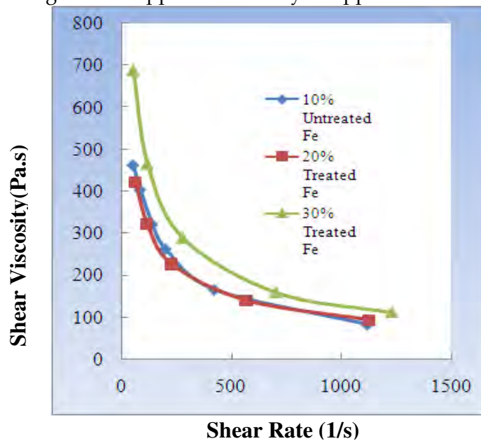
Figure 6-6: Corrected viscosity vs shear rate
