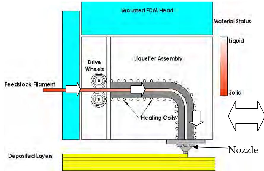
Figure 7-2: Fused Deposition Modelling process in FDM3000
