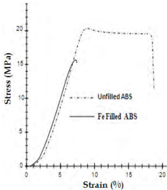
Figure 5-6: Stress-strain behaviour of 10wt% Iron filled ABS and virgin ABS used in FDM
