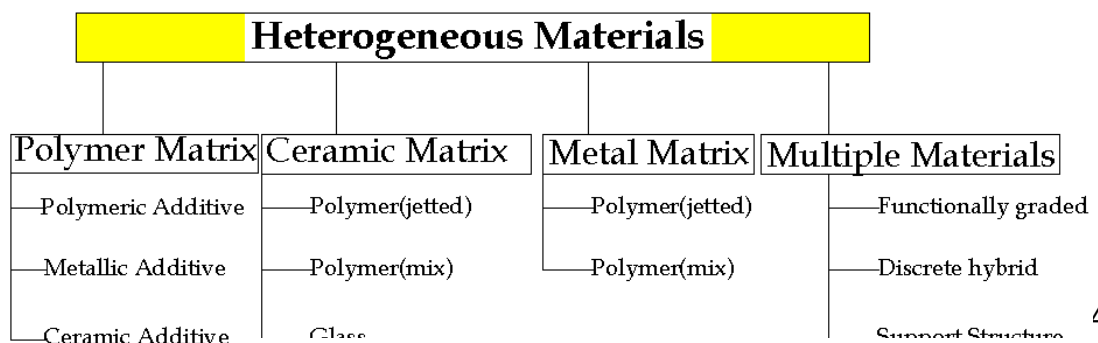
Figure 2-19: A hierarchy of heterogeneous materials system for additive manufacturing (Markforged Ex. 1009)
