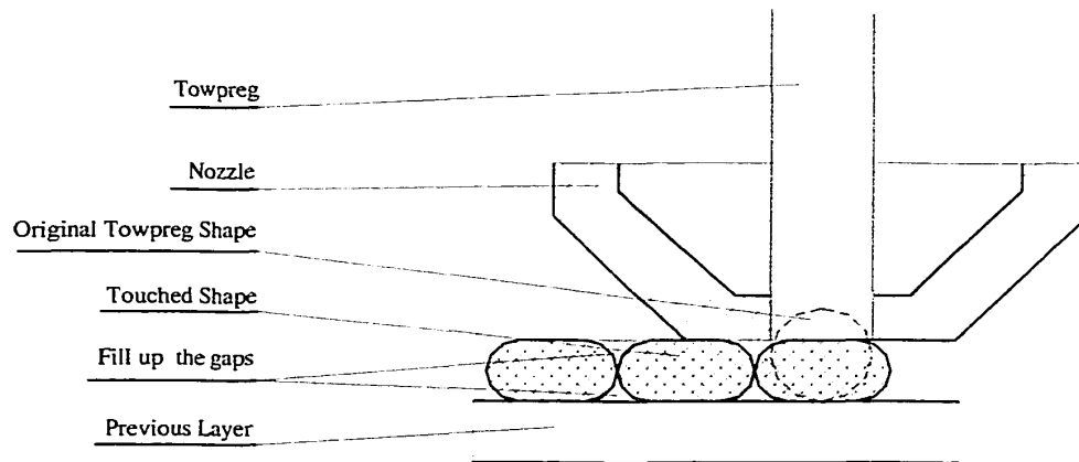
Fig 2-3 Materials distribution. the towpreg shape has been changed during the deposition process.
