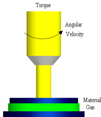
Figure 4-5: Parallel Plate Rheometry
