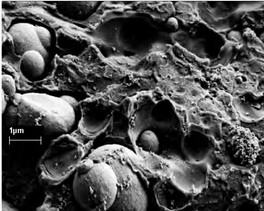
Figure 5-14: SEM image of fracture surface ABS-Fe(20 vol%) prepared by melt compounding
