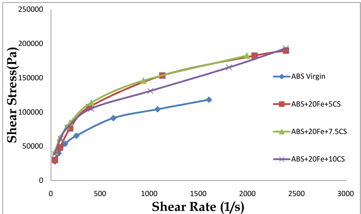
Figure 4-14: Flow curves of composites of ABS and varying volume fractions of Ca.St. in 20% filled iron with particle size <10um
