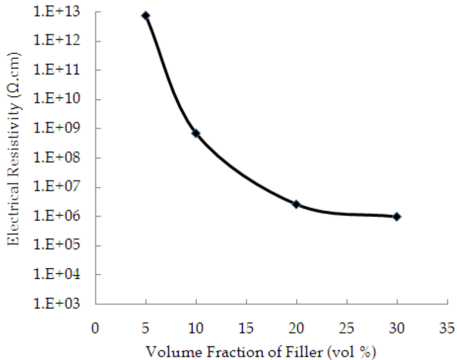
Figure 5-35: DC resistivity of Iron/ABS composites for filler concentration up to 30vol%
