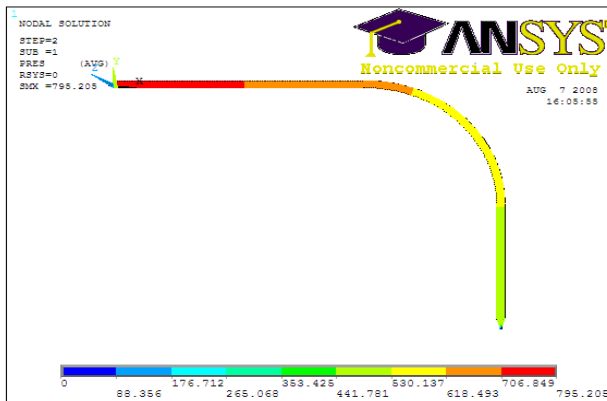
Figure 6-18: pressure drop calculated using Flotran
