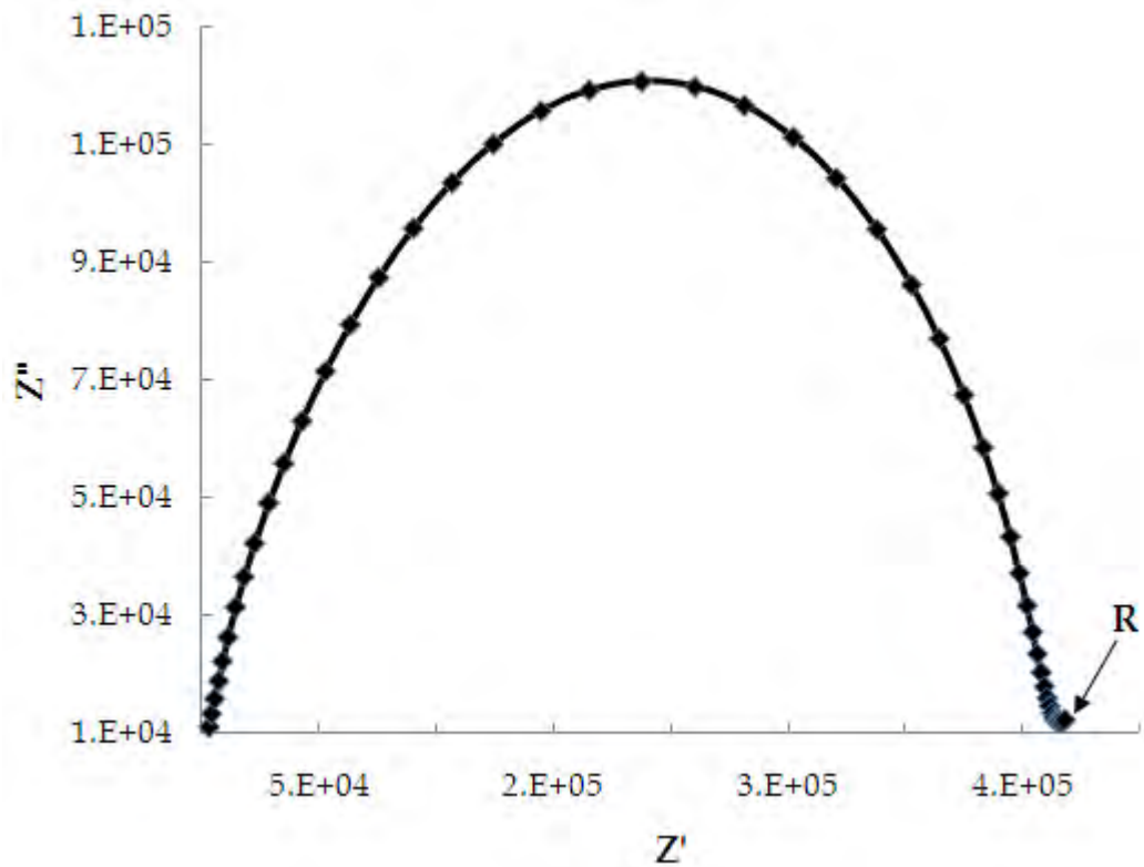
Figure 5-33: Nyquist plot of a Low-filled ABS Composite below Glass Transition Temperature
