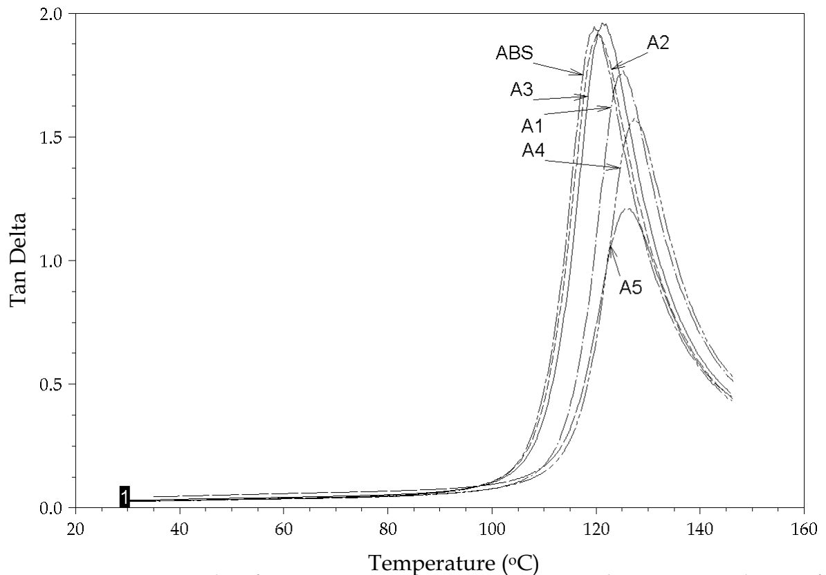
Figure 5-19: Tan Delta of Various Copper/ABS Composites with copper particle size of 10 \mu\text{m} at Temperature Scan
