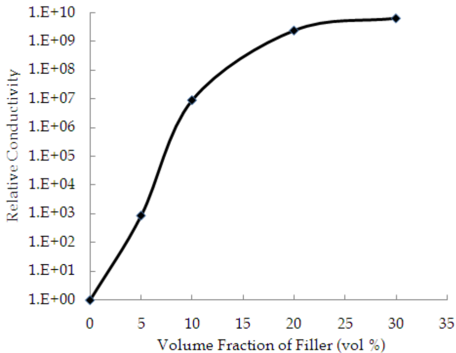
Figure 5-36: Relative DC conductivity of Iron/ ABS composites for filler concentration up to 30 vol%
