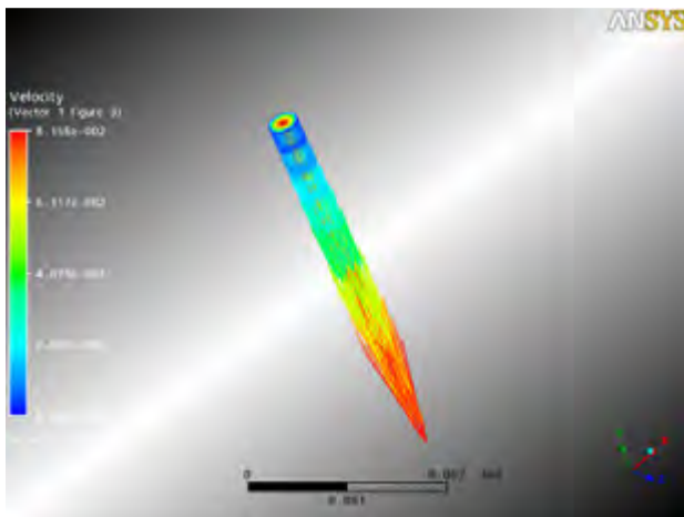
Figure 6-26: Max. Velocity vector at nozzle exit obtained by CFX
