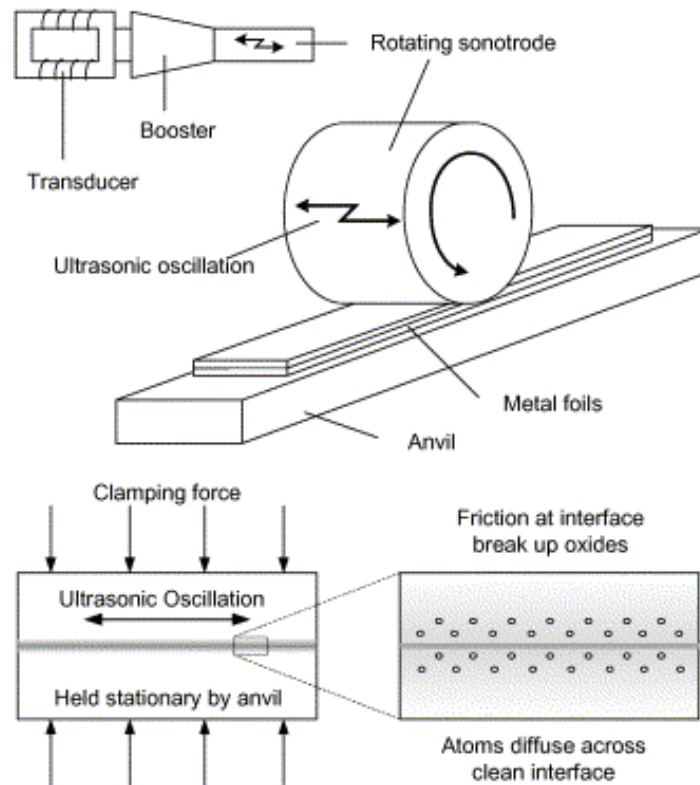
Figure 2-16: Ultrasonic Consolidation of Metal-Matrix Composites (Kong, Soar & Dickens 2004)
