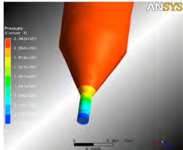
Figure 6-25: Maximum pressure drop at nozzle exit
