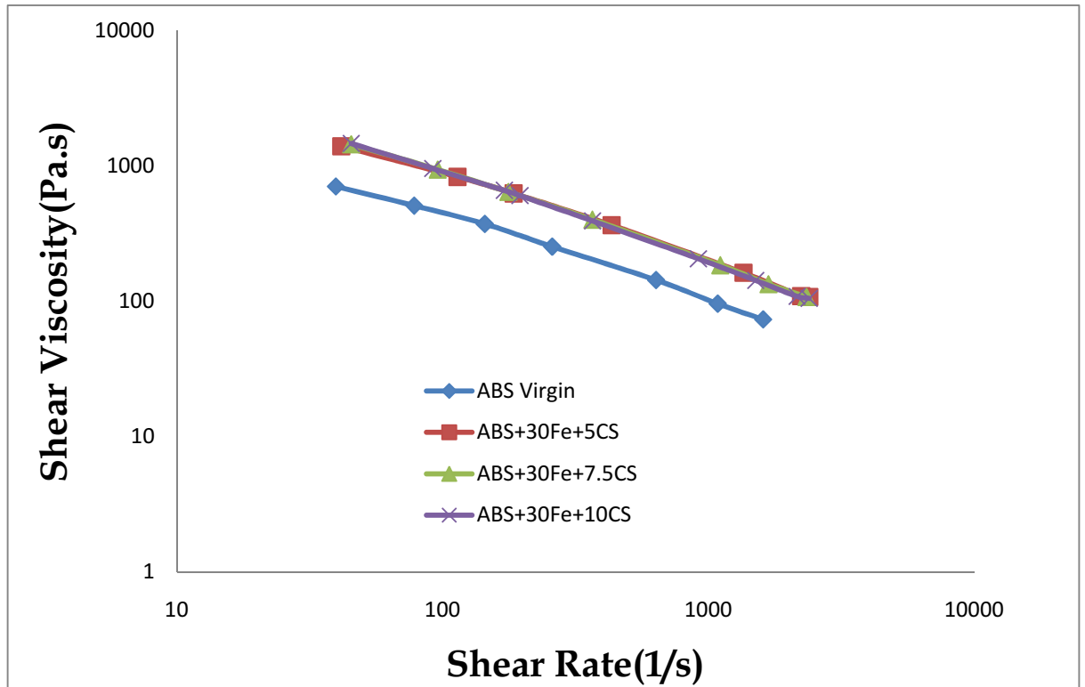
Figure 4-17: Shear rate versus viscosity of various compounds of ABS and Ca.St in 30% filled iron with particle size <10um
