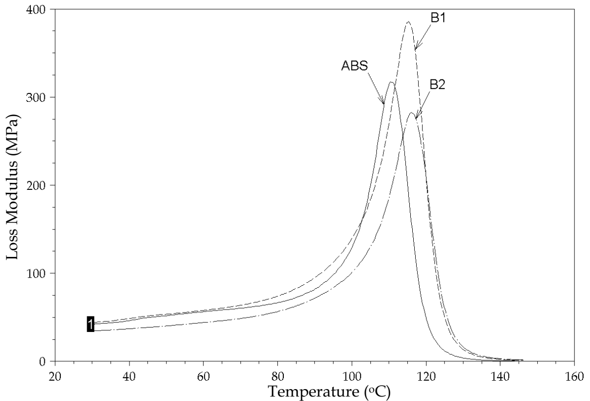
Figure 5-21: Loss Modulus of Various Copper/ABS Composites with copper particle size of 45µm at Temperature Scan
