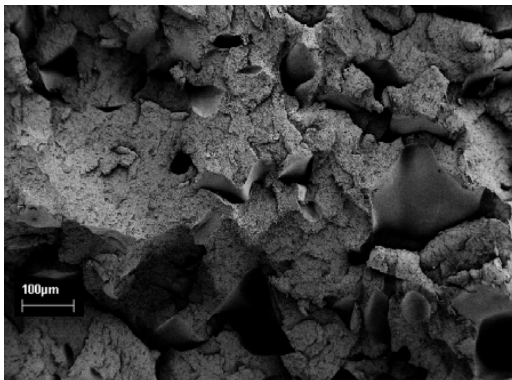
Figure 5-9: Fracture surface of re-processed FDM ABS P400
