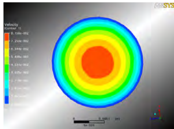
Figure 6-27: Velocity distribution at centre cross section of the tip nozzle tip
