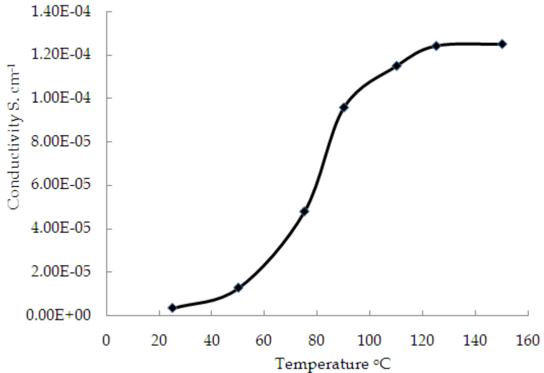
Figure 5-34: Effect of temperature on ionic conductivity of Iron/ABS composites with low iron content
