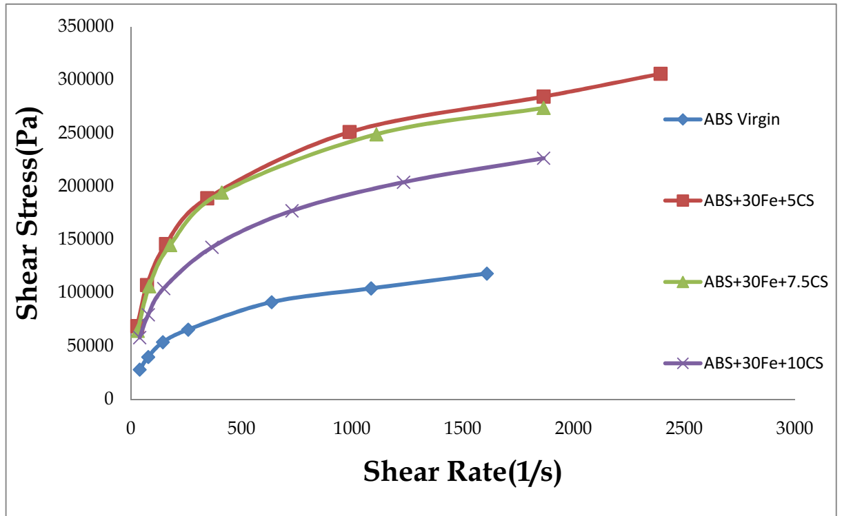
Figure 4-22: Flow curves of composites of ABS and varying volume fractions of Ca.St. in 30% filled iron with particle size <45um
