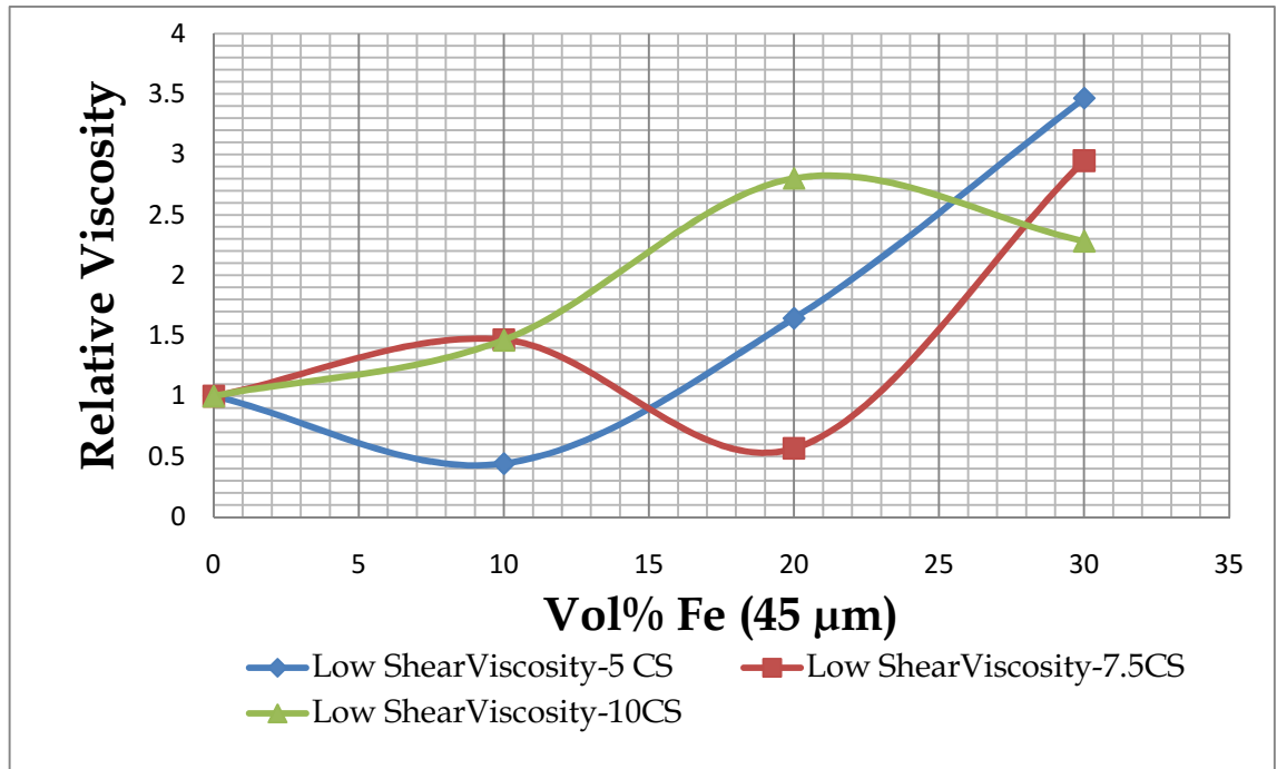
Figure 4-30: Relative viscosity of composites of ABS and varying volume fractions of Ca.St for low shear rate with iron particle size of 45 \mu\text{m}
