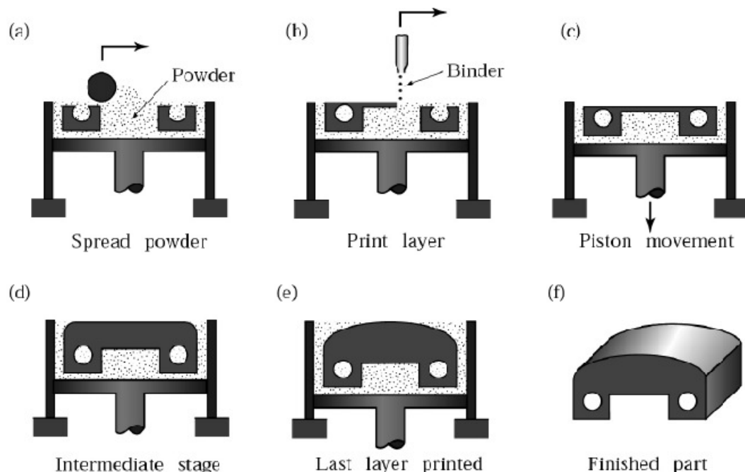
Figure 2-7: Illustration of 3DP process (Source: after E.Sachs and E.Cima)
