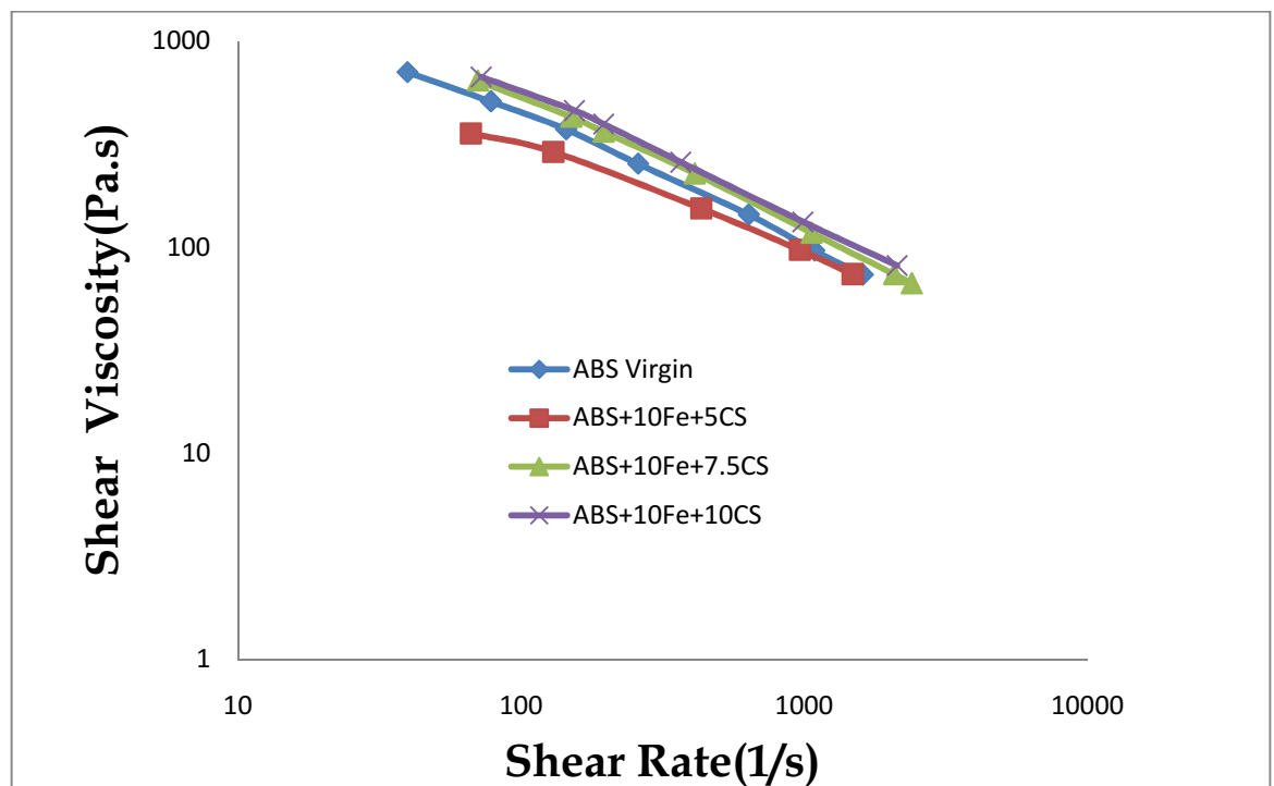
Figure 4-19: Shear rate versus viscosity of various composites of ABS and Ca.St in 10% filled iron with particle size <45um
