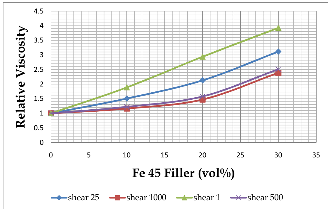
Figure 4-11: Relative viscosity of composites of ABS and varying volume fractions of 45 \mu\text{m} iron
