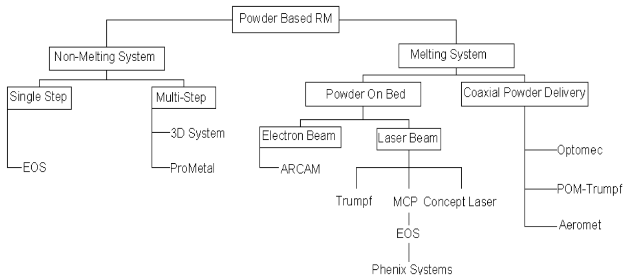
Figure 2-12: Powder-based RM Processes and the Current Commercial Providers (Santos et al. 2006)
