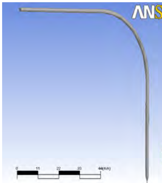
Figure 6-13: 3D mesh of the melt channel
