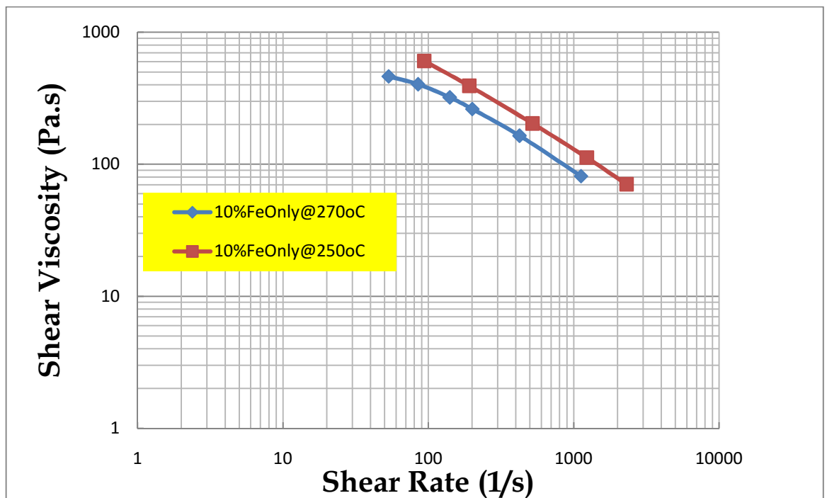
Figure 4-35: Effect of processing temperature on the viscosity of ABS P400
