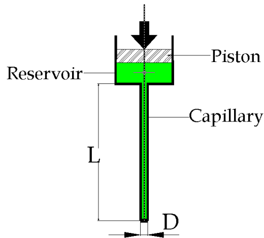
Figure 4-3: Capillary Viscometer
