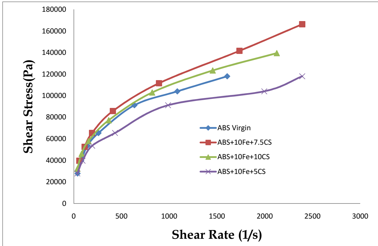
Figure 4-12: Flow curves of composites of ABS and varying volume fractions of Ca.St. in 10% filled iron with particle size <10um
