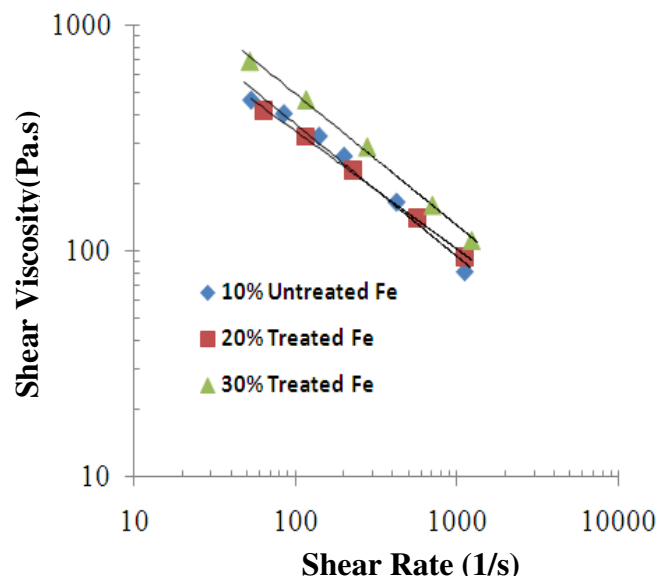
Figure 6-8: Characteristics flow curves plotted to determine flow indices
