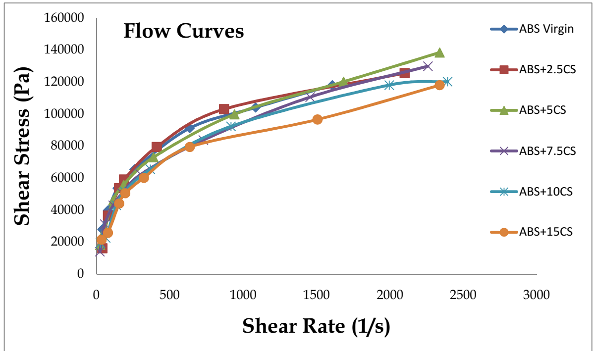
Figure 4-8: Flow curves of composites of ABS and varying volume fractions of Ca.St.
