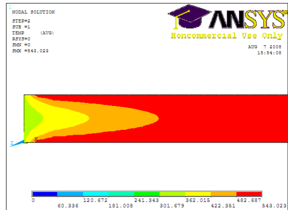
Figure 6-17: Temperature profile of melt at the channel inlet
