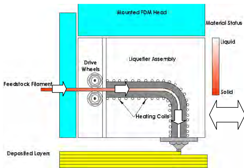
Figure 2-9: Fused Deposition Modelling process
