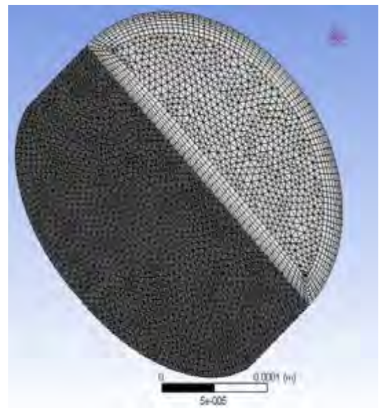
Figure 6-14: Close-up of 3D mesh at Nozzle Tip
