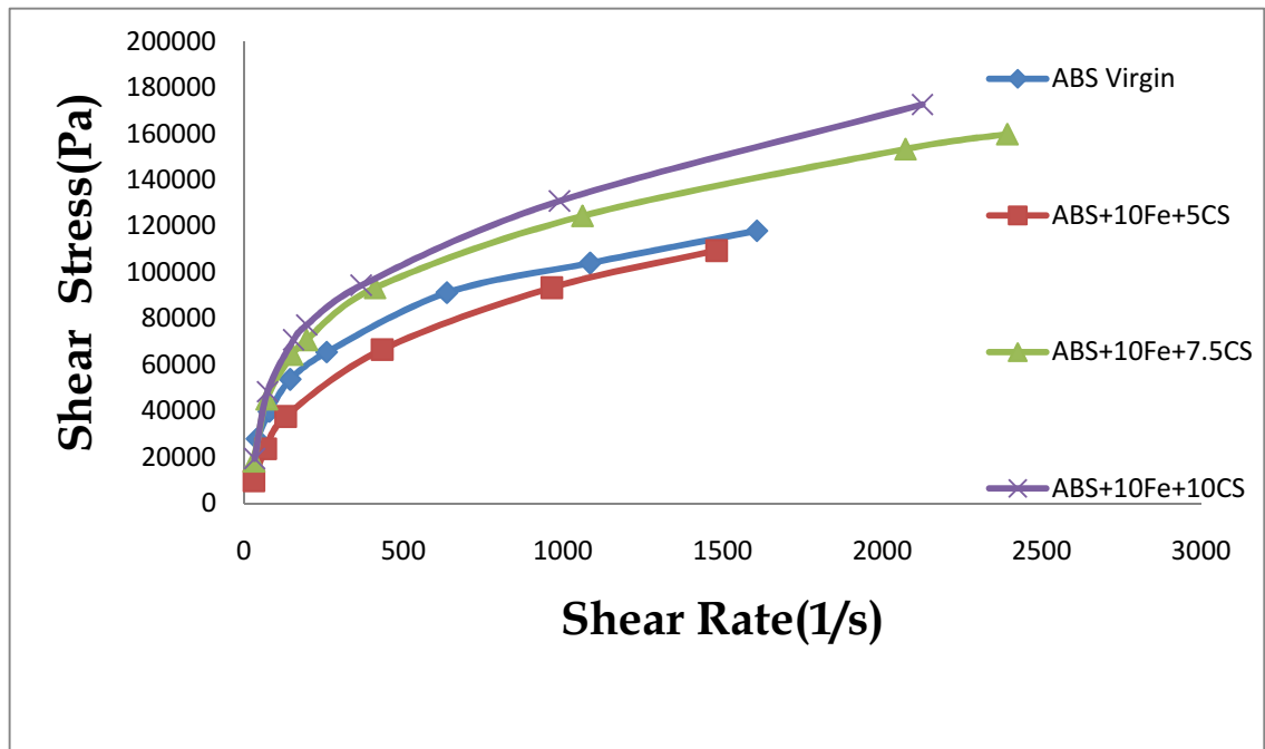
Figure 4-18: Flow curves of composites of ABS and varying volume fractions of Ca.St. in 10% filled iron with particle size <45um
