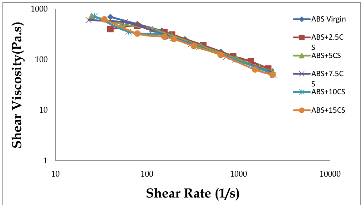
Figure 4-9: Effect of shear rate on the viscosity of various composites of ABS and Ca.St
