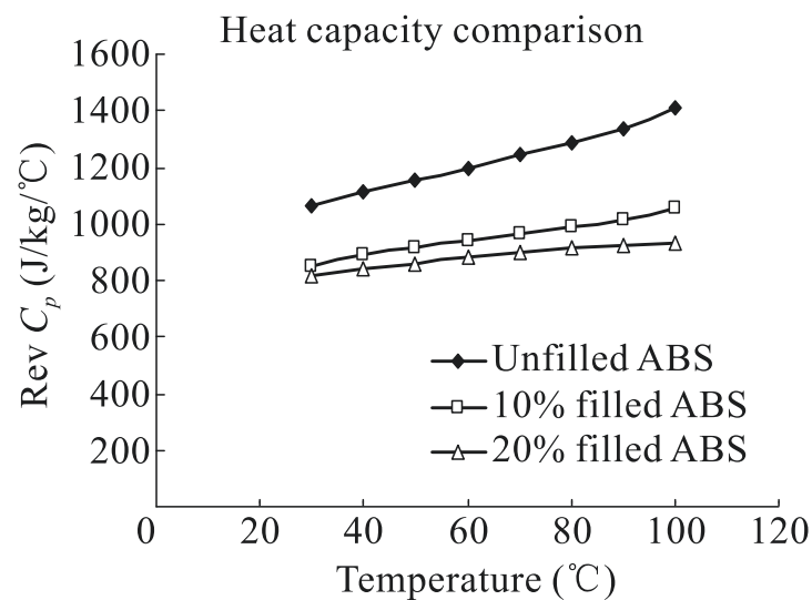
Figure 6-4: Rev Cp of the filled ABS used for thermal conductivity calculation
