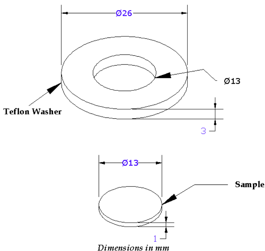
Figure 5-30: Specifications of test sample for Impedance Spectroscopy
