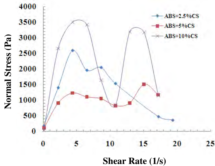
Figure 4-36: Normal Stress versus Shear Rate for ABS with varying %vol of Ca.St.
