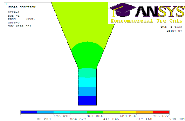
Figure 6-19: pressure drop at nozzle tip
