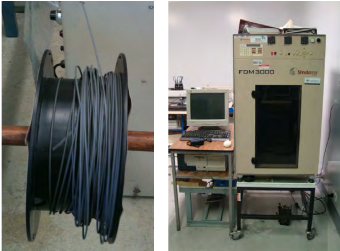
Figure 7-1: (a) Spool of Iron/ABS composite filament and (b) Stratasys FDM 3000
