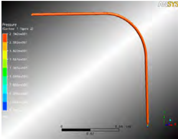
Figure 6-24: Pressure drop along the melt channel in the liquefier head calculated using CFX
