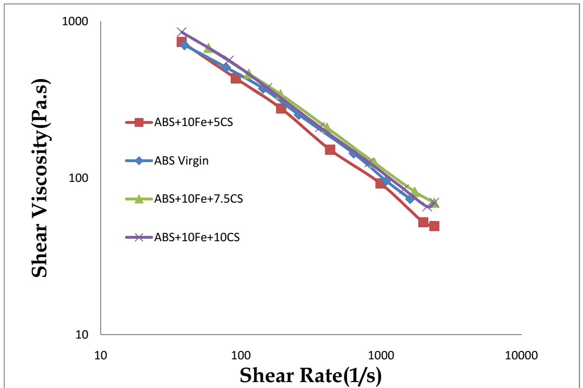
Figure 4-13: Shear rate versus viscosity of various composites of ABS and Ca.St in 10% filled iron with particle size <10um
