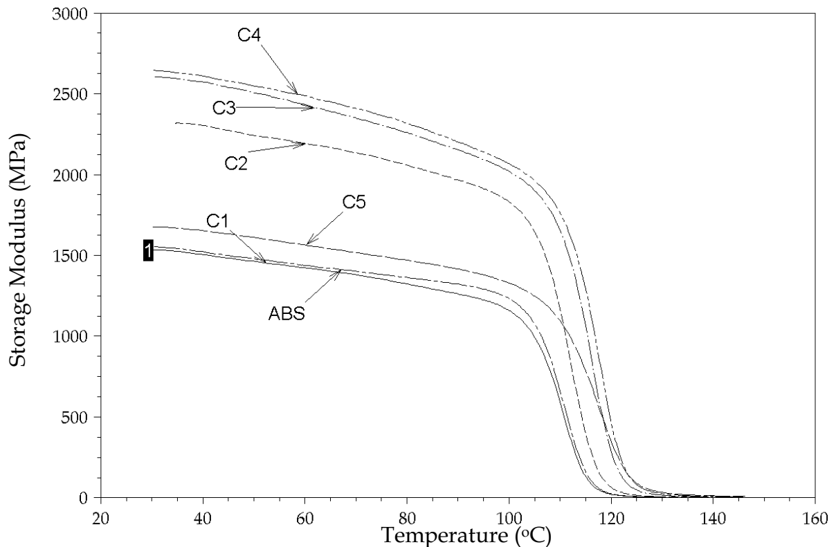
Figure 5-22: Storage Modulus of various Iron/ABS Composites with iron particle size of 45 \mu\text{m} at Temperature Scan
