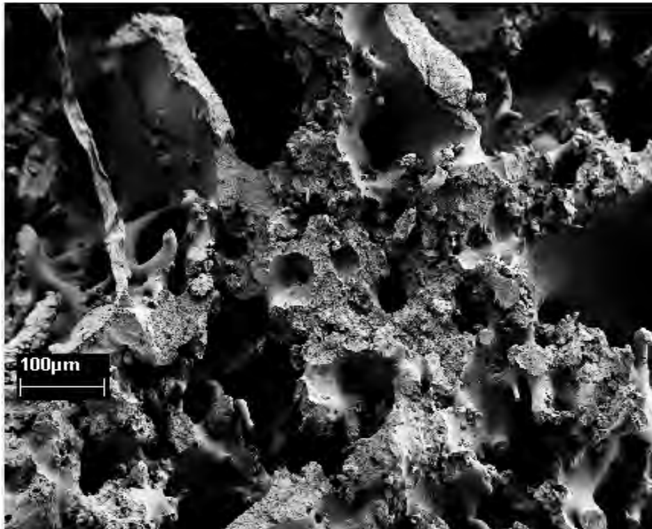
Figure 5-10: SEM image of fracture surface ABS-Fe(10 vol%)prepared via centrifugal mixing
