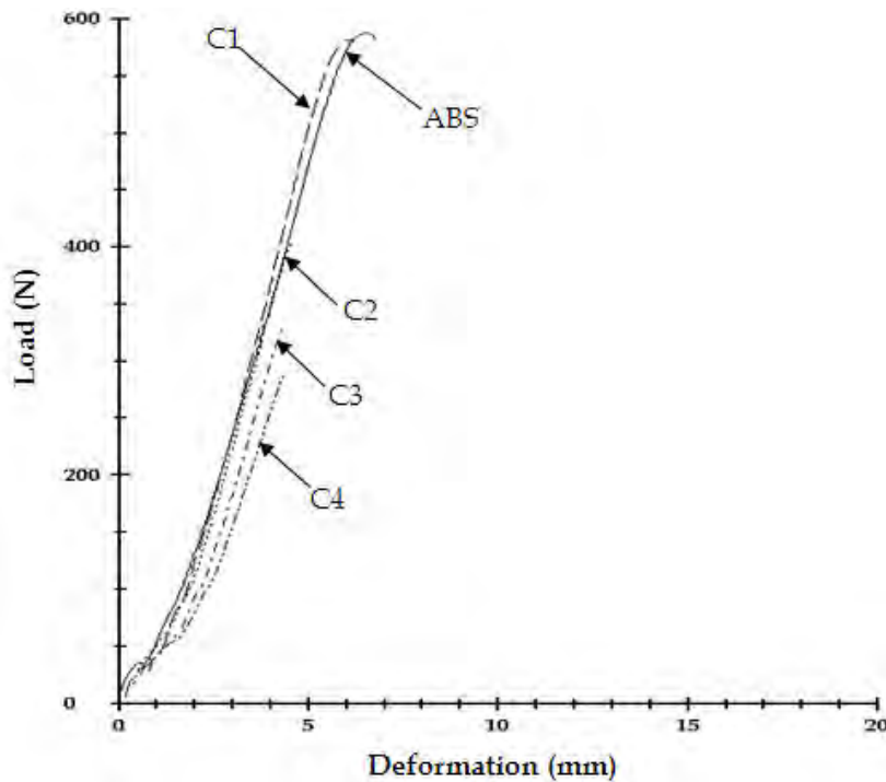
Figure 5-5: Load vs deformation behaviour of Iron/ABS composites prepared by centrifugal mixing with various volume fractions of Iron powder
