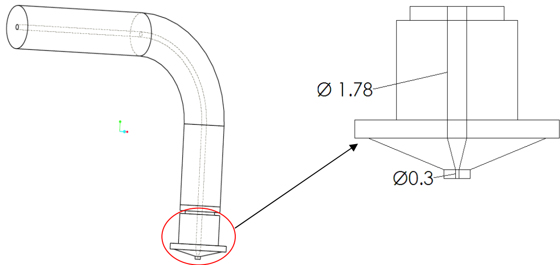
Figure 6-1: (a). Schematic of FDM Liquefier, (b). FDM Tip Nozzle Configuration
