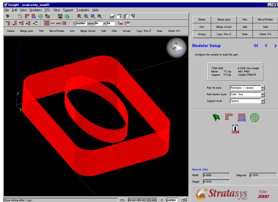
Figure 7-7: Sliced model of the tooling insert for creation of tool paths
