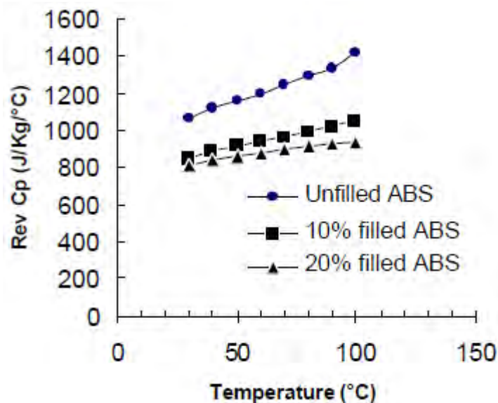
Figure 5-29: Rev Cp of the iron filled ABS composites
