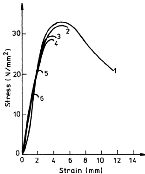
Figure 5-2: Stress-strain curves for HDPE/zinc composites with different concentrations of zinc powder: 0% vol (1); 4% vol (2); 8% vol (3); 12% vol (4); 16% vol (5); 20% vol (6) (Sofian & Rusu 2001)
