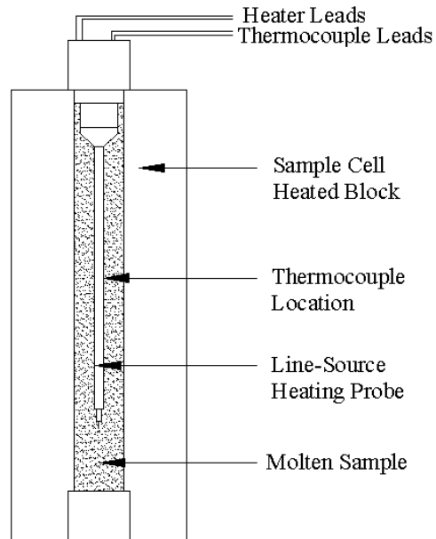
Figure 5-26: Schematic of Thermal Conductivity Apparatus
