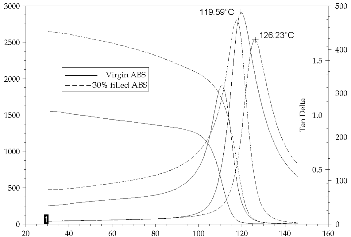
Figure 5-25: Comparison of dynamic mechanical properties of virgin ABS and 30 % iron-powder filled ABS
