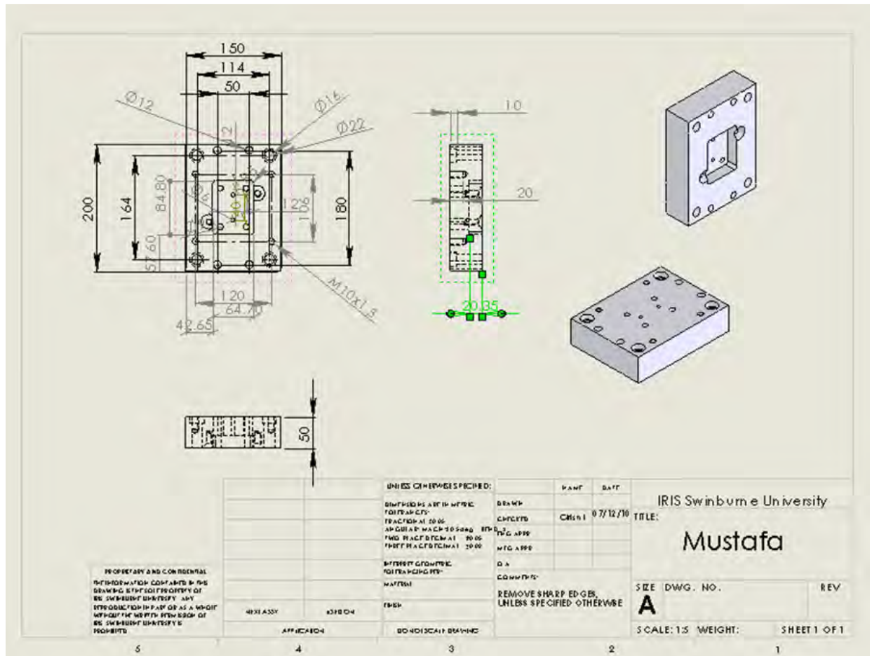
Figure 7-11: Drawing detail of injection blade as the backing for tooling insert
