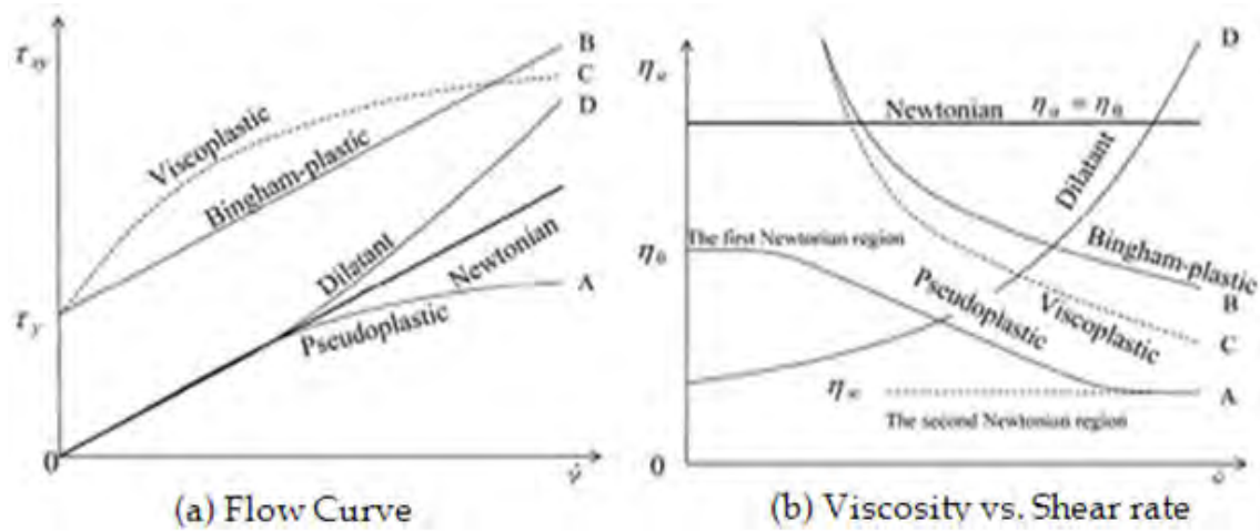
Figure 6-7: (a) Characteristics flow curves, and (b) viscosity vs shear rate for non-Newtonian fluids (Yamaguchi)
