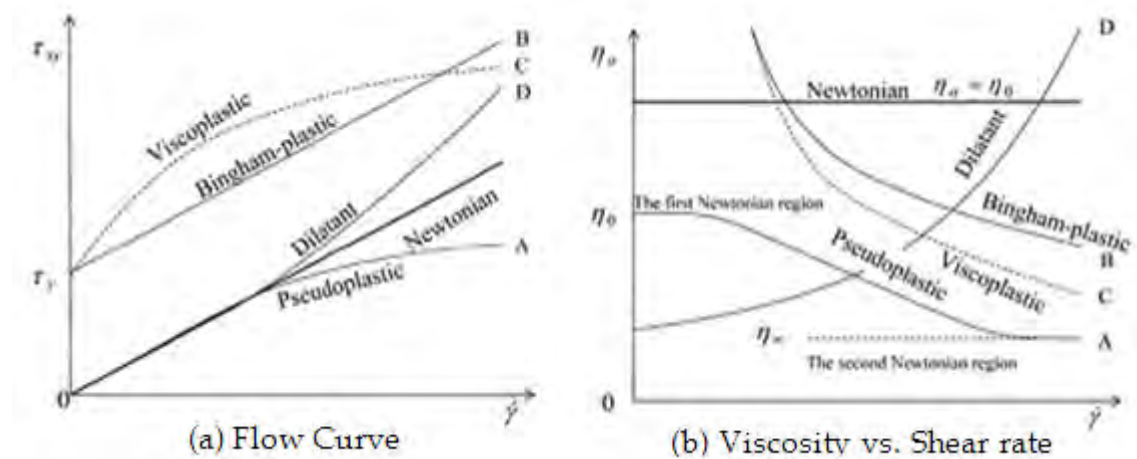
Figure 4-2: Pure viscous non-Newtonian fluids (Yamaguchi 1952)
