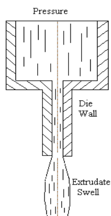
Figure 3-5: Schematic of Polymer Melt Swell
