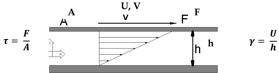
Figure 4-1: Simple Shear Flow
