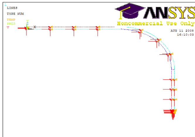
Figure 6-15: Boundary conditions set for thermo-fluid analysis of the FDM3000 melt flow channel
