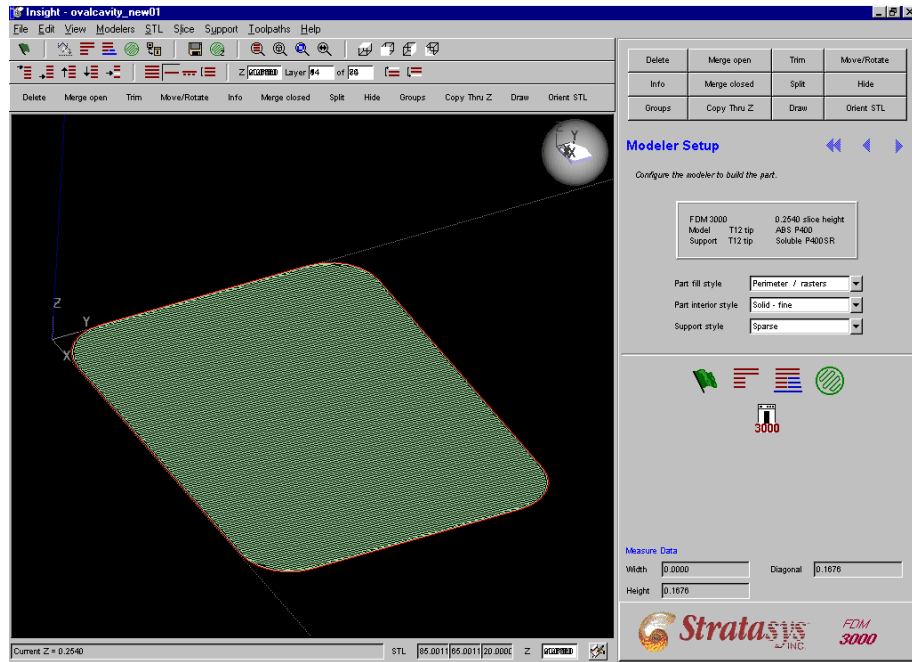
Figure 7-8: A criss-cross fill pattern for the bottom layer of the model
