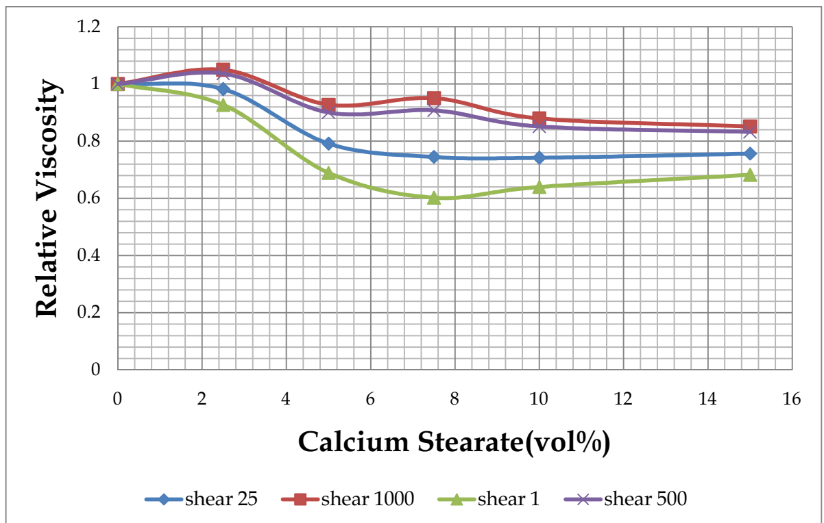
Figure 4-10: Relative viscosity of composites of ABS and varying volume fractions of Ca.St. at different shear rates
