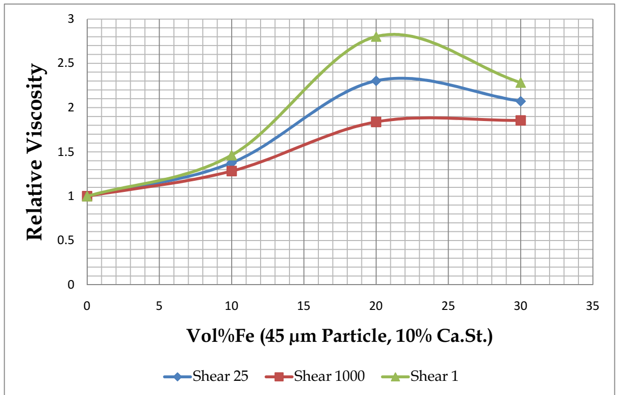
Figure 4-26: Relative viscosity of composites of ABS and varying volume fractions of Fe of 45 μm and 10%Ca.St.
