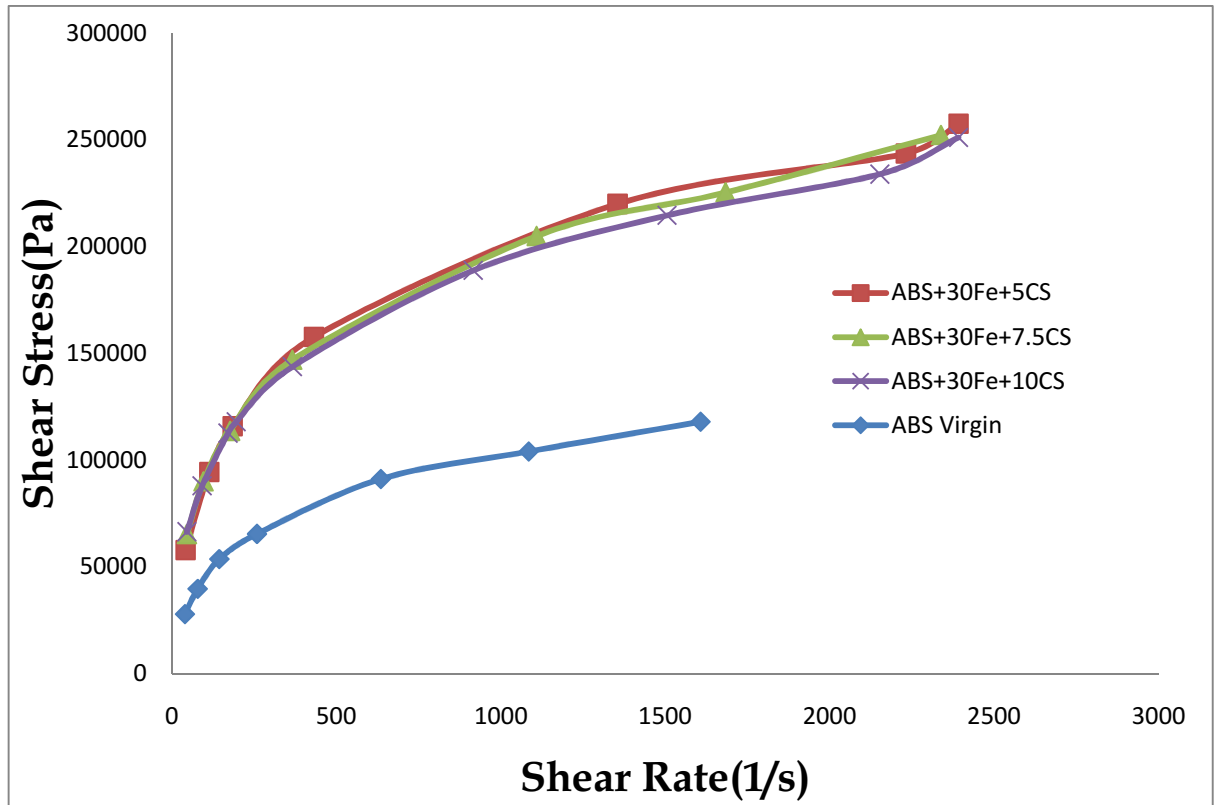
Figure 4-16: Flow curves of composites of ABS and varying volume fractions of Ca.St. in 30% filled iron with particle size <10um
