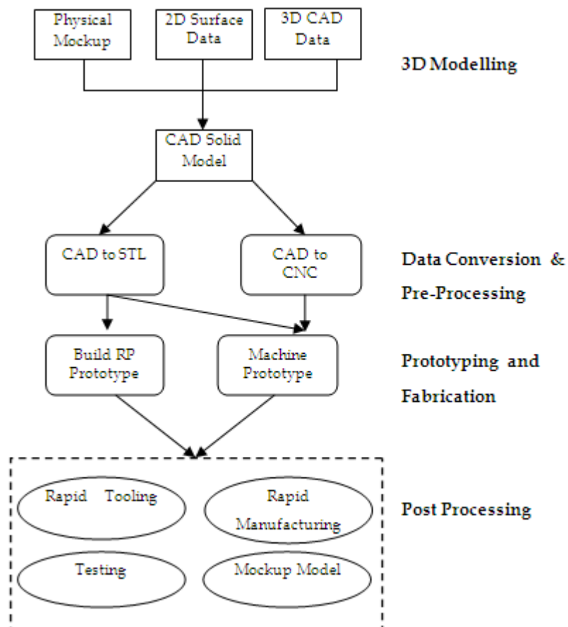
Figure 1-1: Generic Flow of RP Process ( Kamrani & Nasr 2006)
