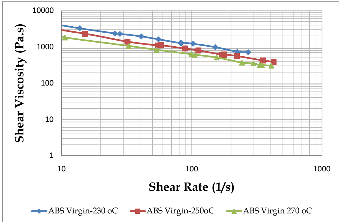
Figure 4-34: Effect of processing temperature on the viscosity of Fe/ ABS composites
