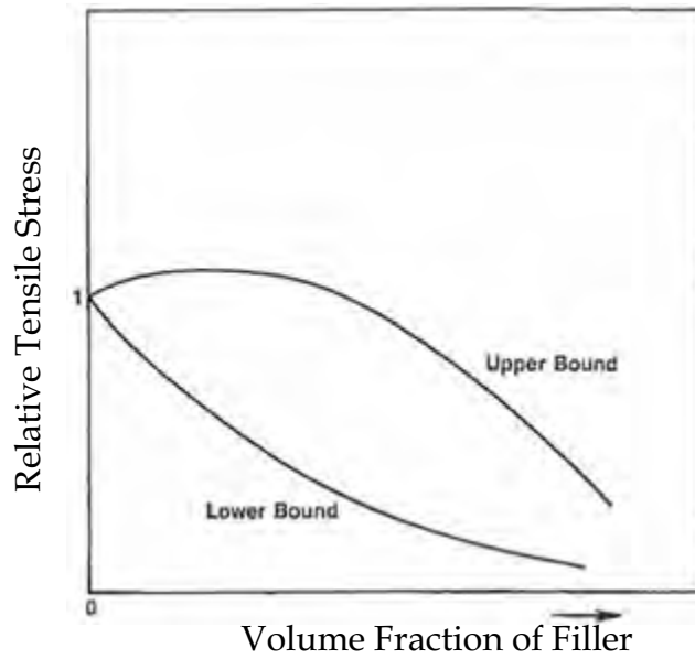
Figure 5-1: Typical tensile stress vs. concentration curves for filled polymers showing upper bound and lower bound responses (Bigg 1987b)
