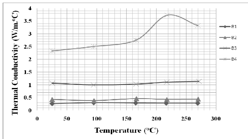
Figure 5-27: Thermal Conductivity of copper filled ABS composites at various temperatures
