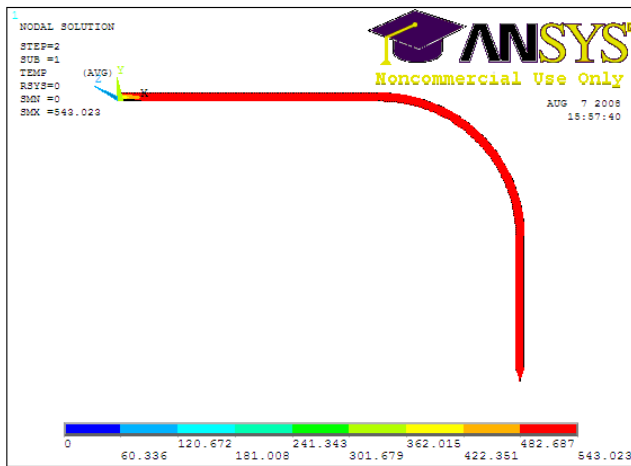
Figure 6-16: Temperature gradient over the melt channel within liquefier
