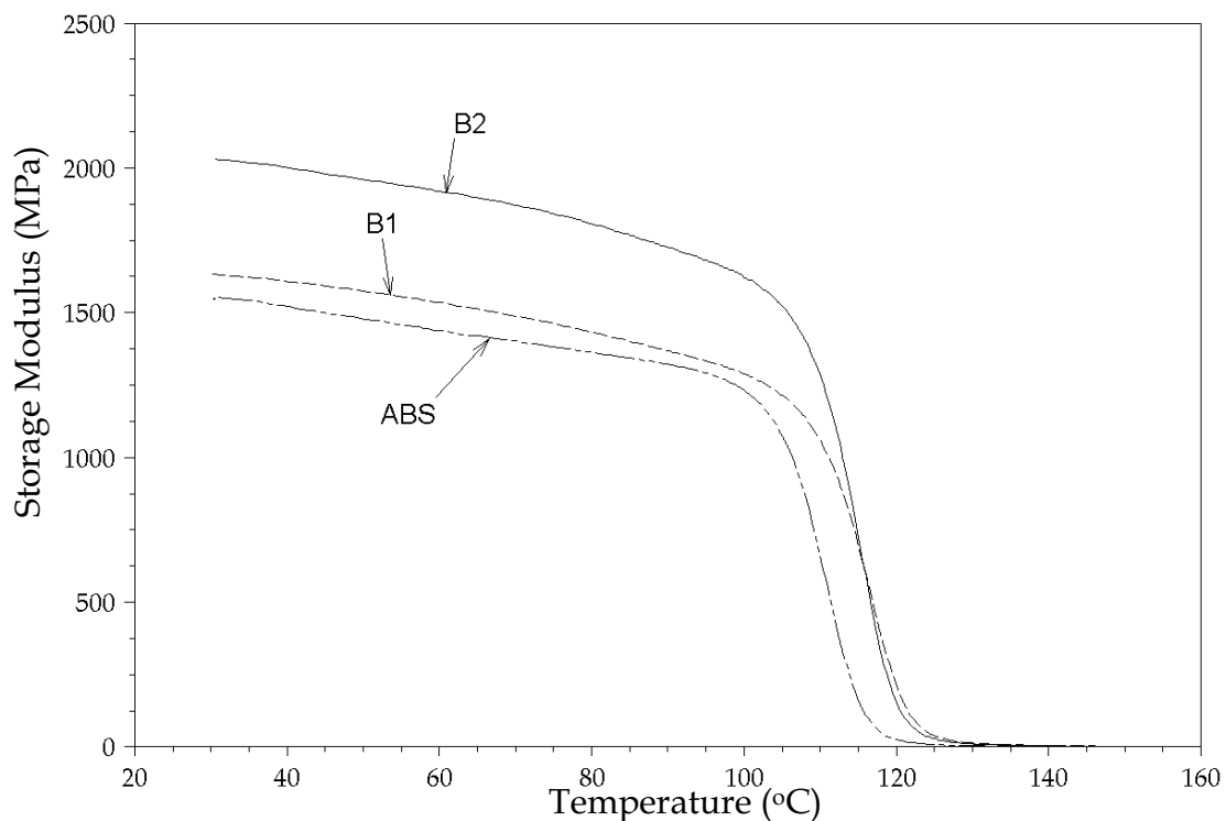
Figure 5-20: Storage Modulus of Various Copper/ABS Composites with copper particle size of 45 \mu\text{m} at Temperature Scan
