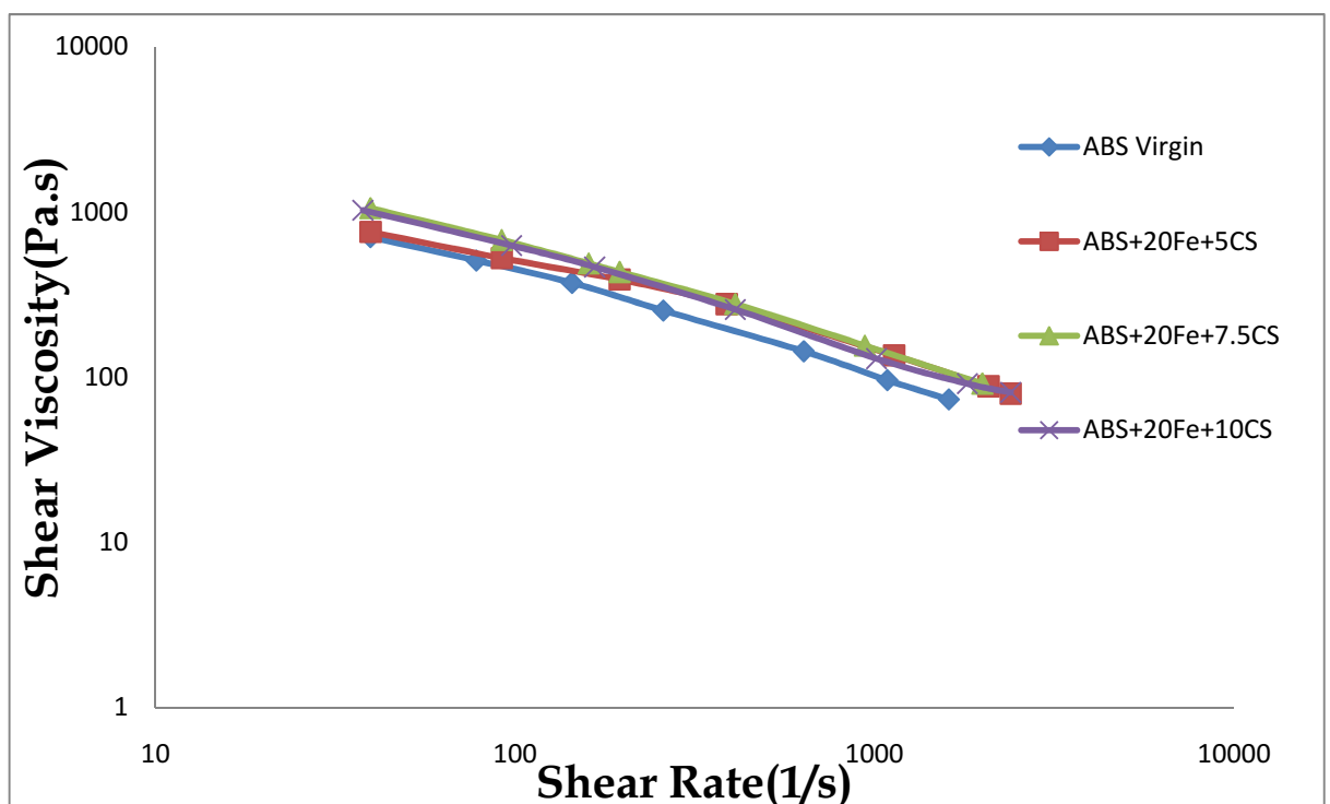
Figure 4-15: Viscosity vs. shear rate for various composites of ABS and Ca.St in 20% filled iron with particle size <10um
