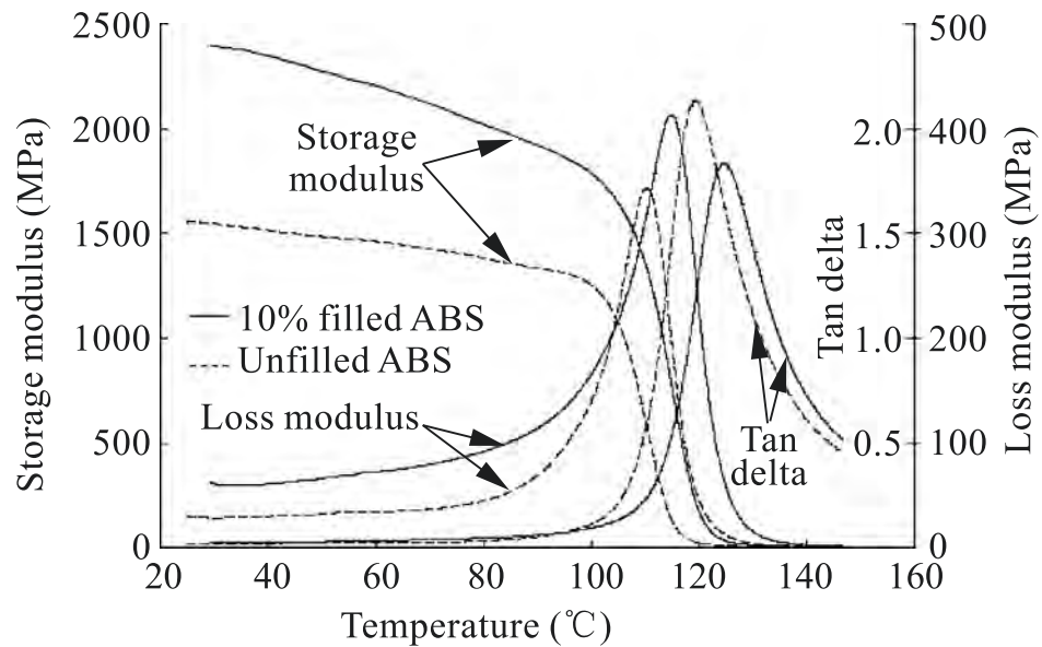
Figure 6-3: Glass transition temperature of 10% Iron filled ABS
