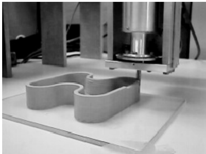
Figure 2-17: Contour Crafting of Structural Ceramic (Khoshnevis et al. 2001)
