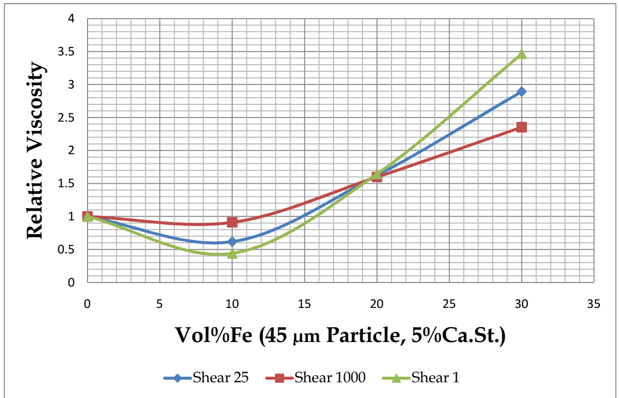
Figure 4-24: Relative viscosity of composites of ABS and varying volume fractions of Fe of 45 μm and 5%Ca.St.
