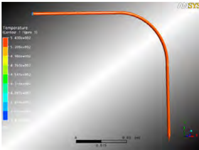
Figure 6-22: 3D Temperature profile along the melt channel in the liquefier head using CFX
