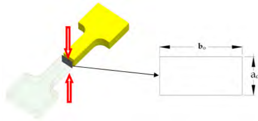
Figure 5-16: Specifications of Tensile Test Sample
