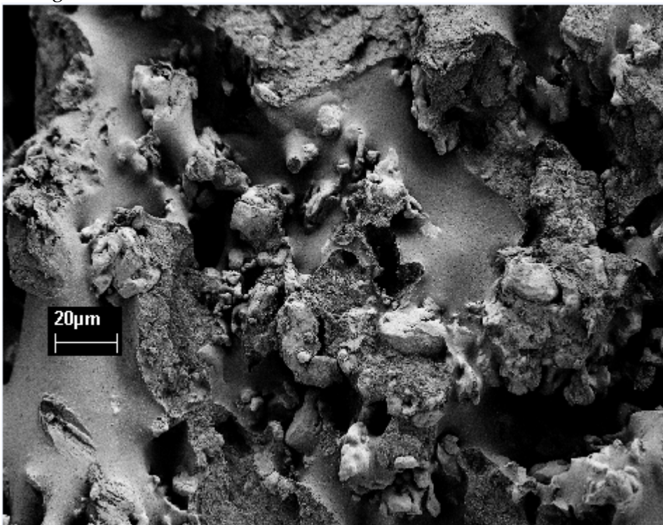
Figure 5-10: SEM image of fracture surface ABS-Fe(10 vol%)prepared via centrifugal mixing
