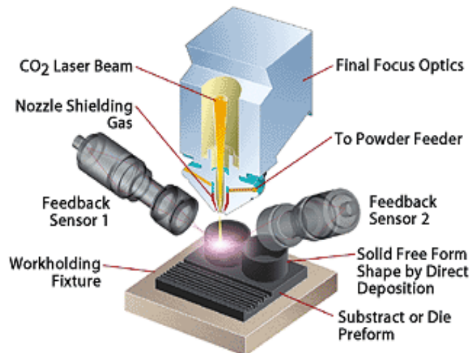
Figure 2-14: Direct Metal Deposition (Courtesy of the POM Group Inc.)
