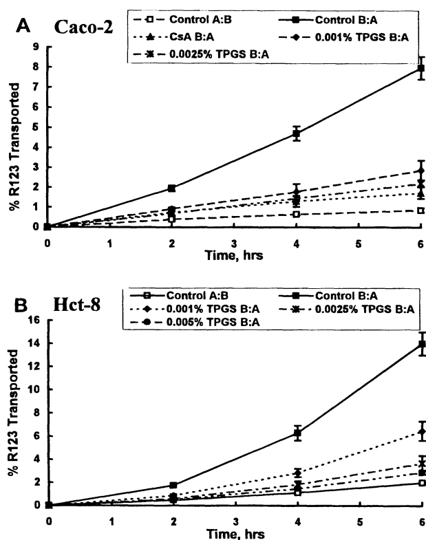
Fig. 6. Rhodamine 123 transport in Caco-2 and HCT-8 cells. Caco-2 ( A ) and HCT-8 ( B ) were grown on Transwell dishes as described in Materials and Methods. Rhodamine 123, 13 \mu\text{M} , was added to the apical or basolateral compartment in the absence or presence of CsA, 5 \mu\text{M} , or 0.0025, 0.005, 0.001% TPGS and media aliquots were taken from the opposite chamber at the indicated times. The data presented are the mean \pm SD of triplicate wells and are representative of at least three independent experiments.
