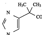
and 4-imidazo- \alpha,\alpha -dimethyl-acetyl
