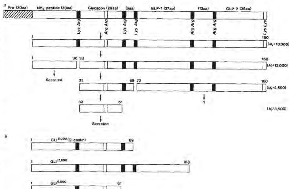
Fig. 3 Schematic representation of the processing of pancreatic preproglucagon and the structure of glucagon-containing polypeptides. a , Possible pathway for the proteolytic processing of pancreatic preproglucagon. The basic dipeptides are indicated and those which are potential sites for cleavage are dark boxes. The numbers in parentheses at the end of each line are the sizes of the glucagon-containing intermediates determined by Patzelt et al. 5 . The numbers above the lines are the amino acids at the ends of the polypeptide in relation to the sequence of preproglucagon (Fig. 1). b , Structure of non-pancreatic glucagon-containing polypeptides. GLI 8,000 and GLI 12,000 are major polypeptides in the intestine and GLI 9,000 accumulates in the serum of animals with renal
