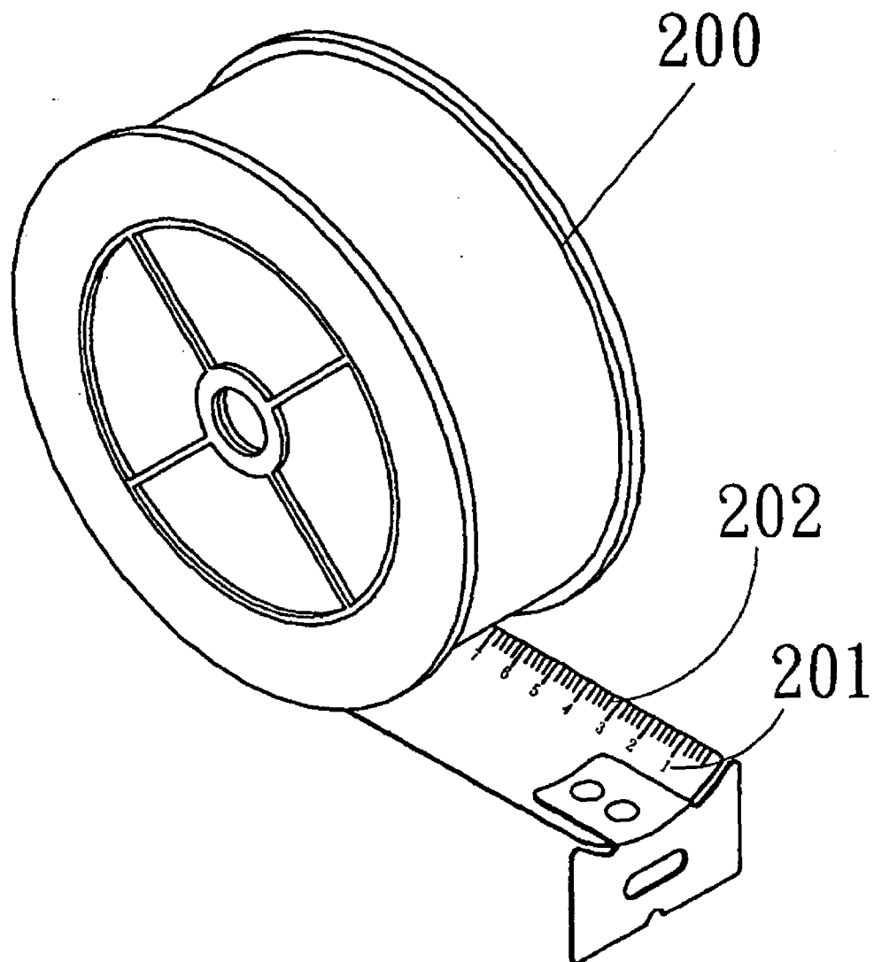
FIG. 2 (PRIOR ART)
