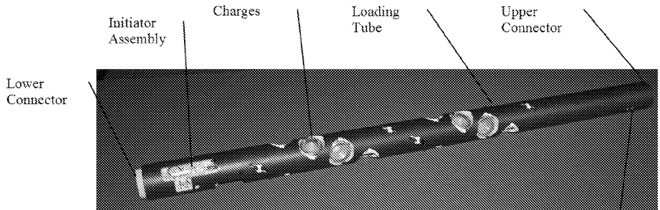
Fig. 2: Fully assembled Steel Loading Tube
