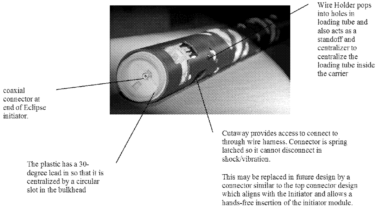
Fig. 5: End of loading tube
