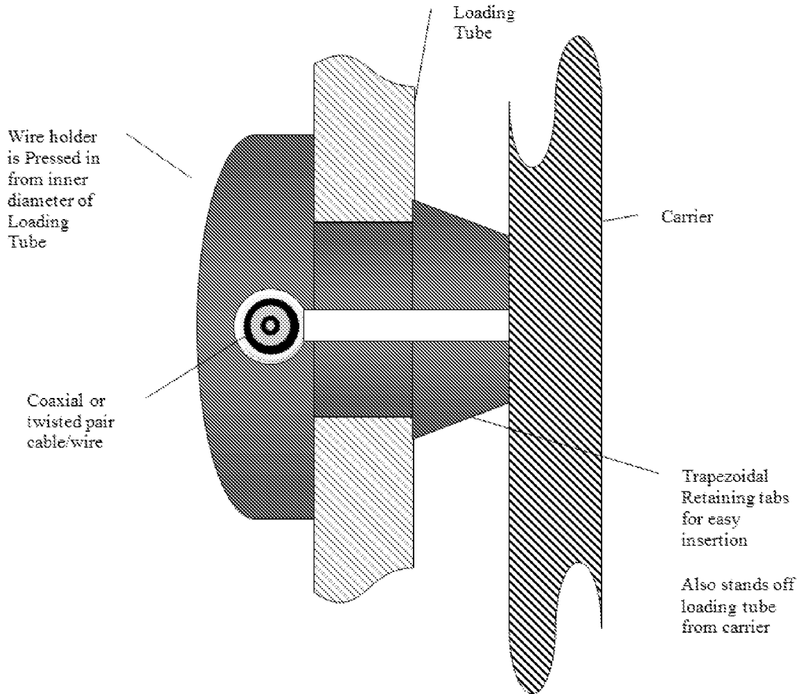
Fig. 6: Example of wire holder
