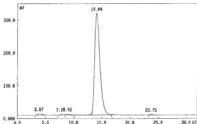
Figure 2. Typical radio-HPLC chromatogram of RP697.
