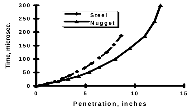
Figure 5 Penetration time-of-arrival
