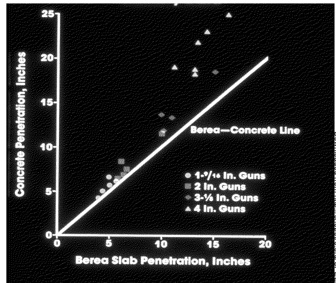
Figure 3 Concrete versus Berea slab penetration data
