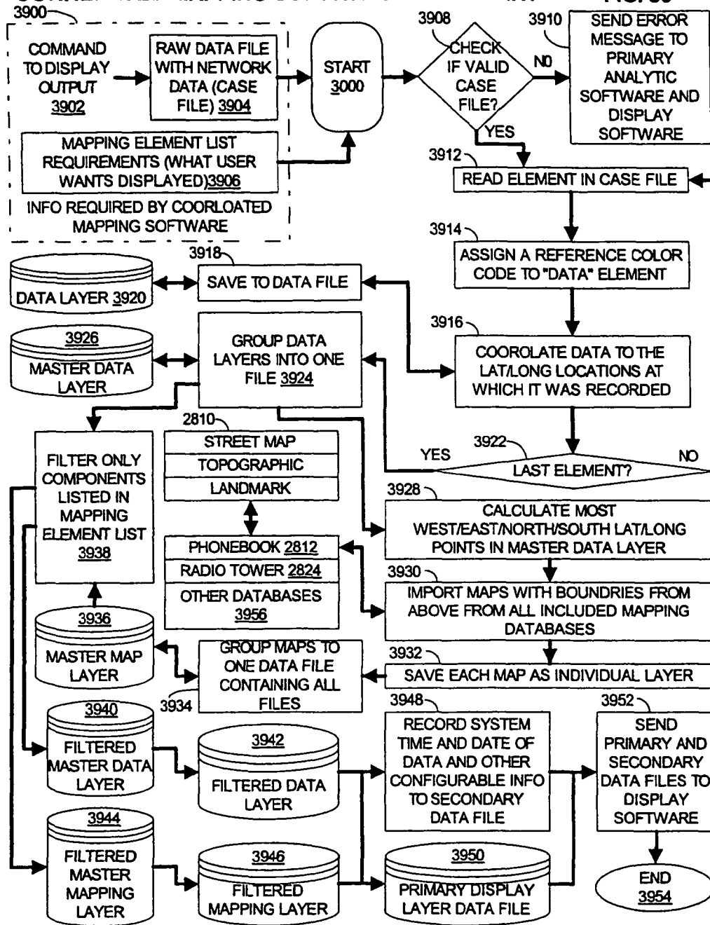
CORRELATED MAPPING SOFTWARE FLOWCHART
